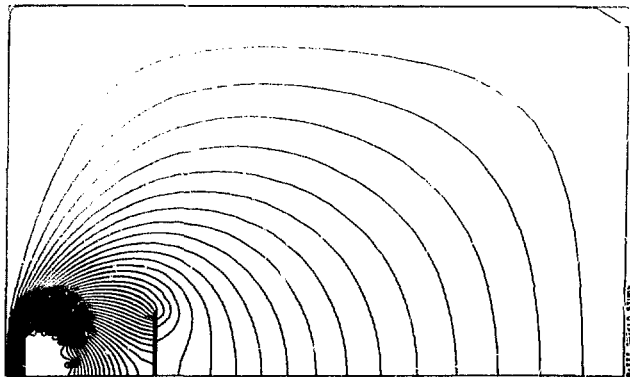
Fig. 11. Flux distribution computed by TRIM for the Doublet-III.
