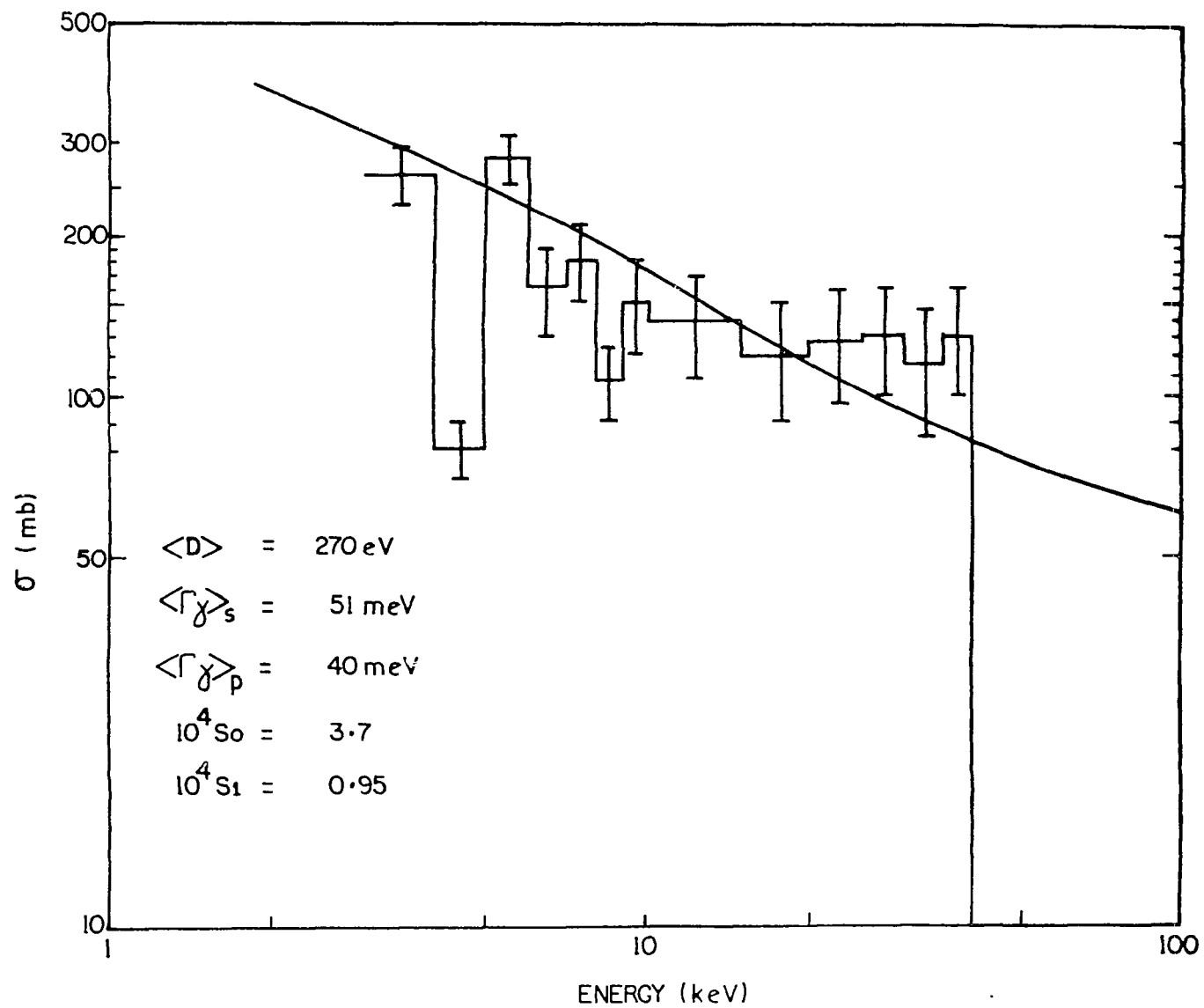
FIGURE 5. CROSS SECTION FOR ^{146}\text{Nd} (n,\gamma) COMPARED WITH STATISTICAL MODEL CALCULATION
