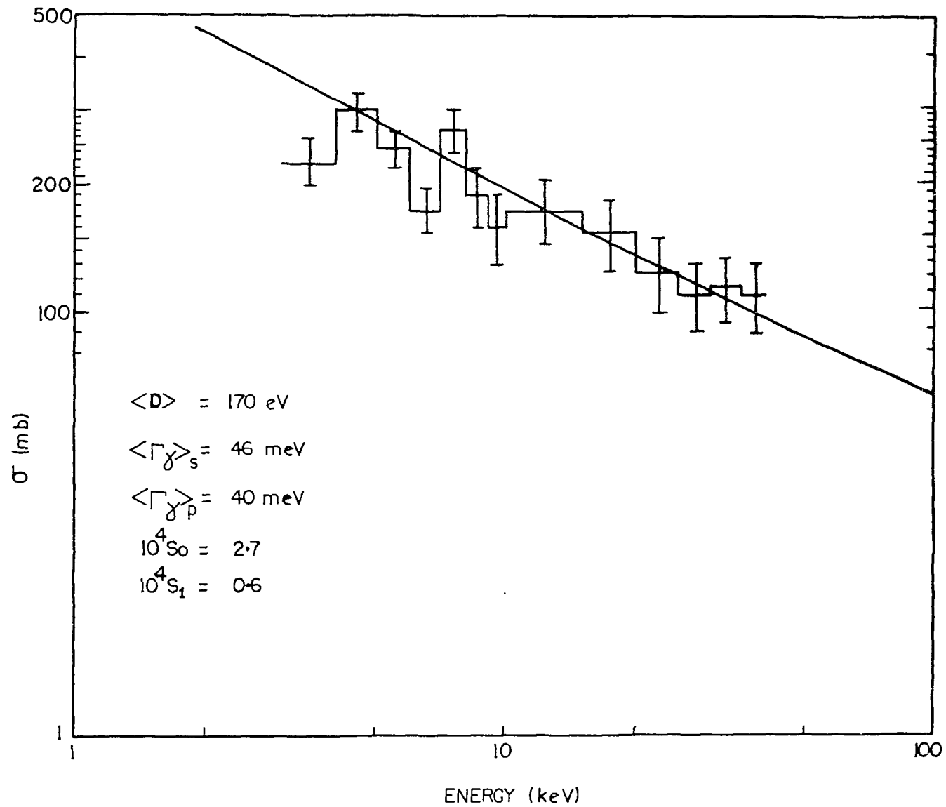
FIGURE 6. CROSS SECTION FOR ^{148}\text{Nd} (n,\gamma) COMPARED WITH STATISTICAL MODEL CALCULATION.
