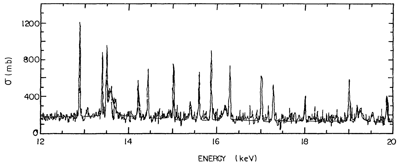
FIGURE 1. FIT TO EXPERIMENTAL DATA FOR ^{142}\text{Nd}(n,\gamma) BETWEEN 12 AND 20 keV.
