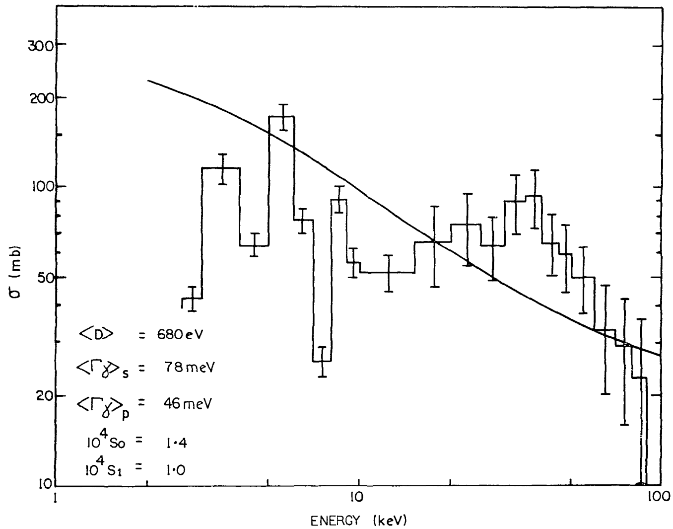
FIGURE 2 . CROSS SECTION FOR ^{142}\text{Nd} (n,\gamma) COMPARED WITH STATISTICAL MODEL CALCULATION
