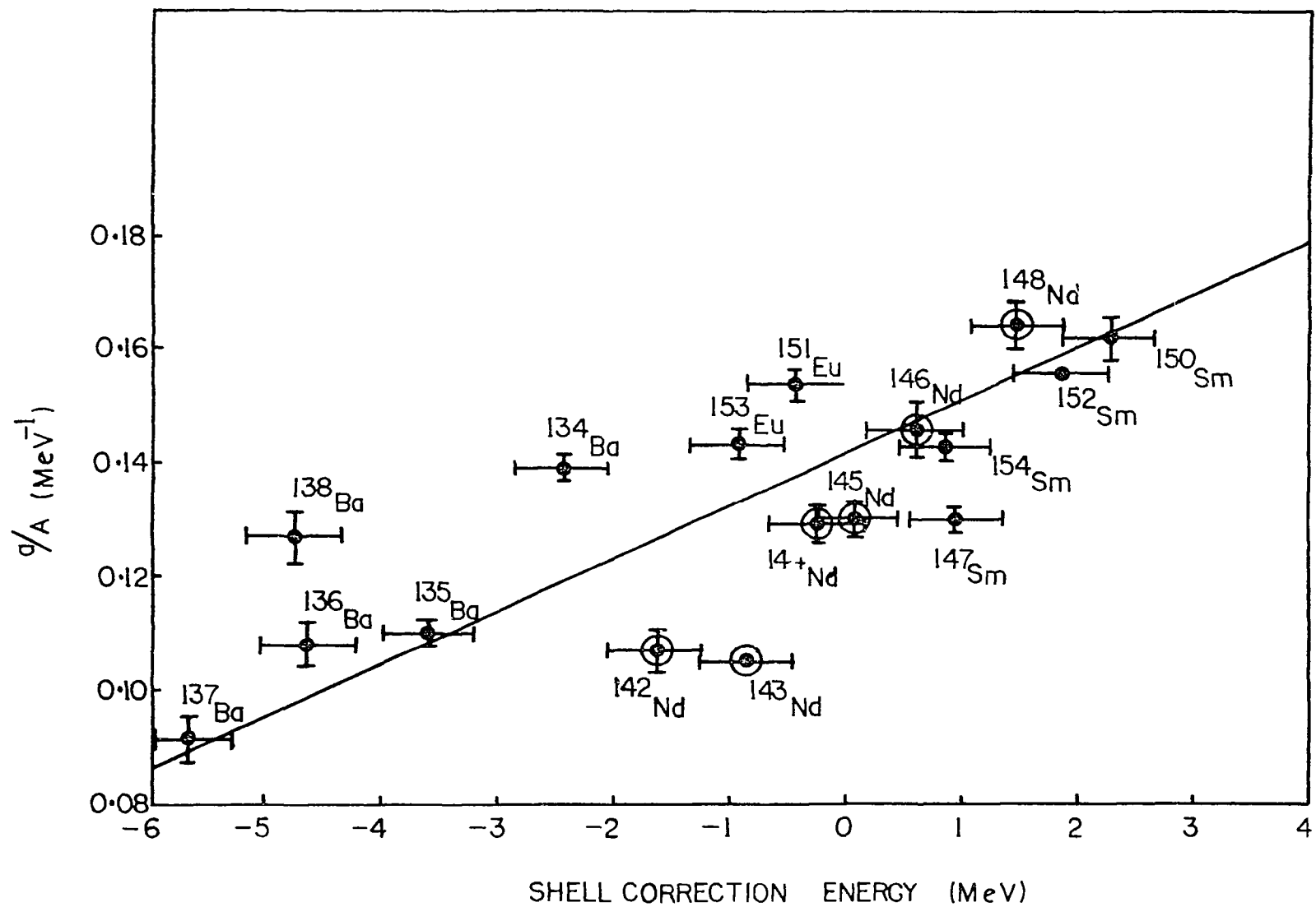
FIGURE 7. LEVEL DENSITY PARAMETER a/A VERSUS THE CAMERON SHELL CORRECTION ENERGY. ALSO SHOWN IS THE GILBERT & CAMERON GLOBAL FIT FOR UNDEFORMED NUCLEI.
