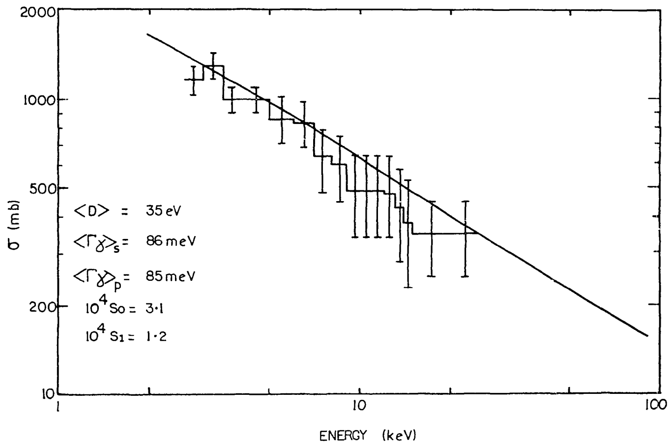
FIGURE 3. CROSS SECTION FOR ^{143}\text{Nd} (n, \gamma ) COMPARED WITH STATISTICAL MODEL CALCULATION
