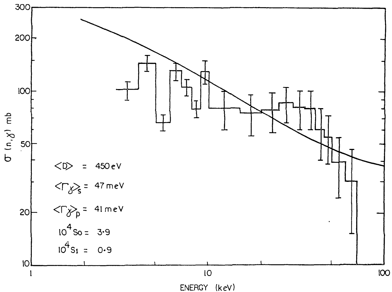
FIGURE 4 . CROSS SECTION FOR ^{144}\text{Nd} (n, \gamma) COMPARED WITH STATISTICAL MODEL CALCULATION
