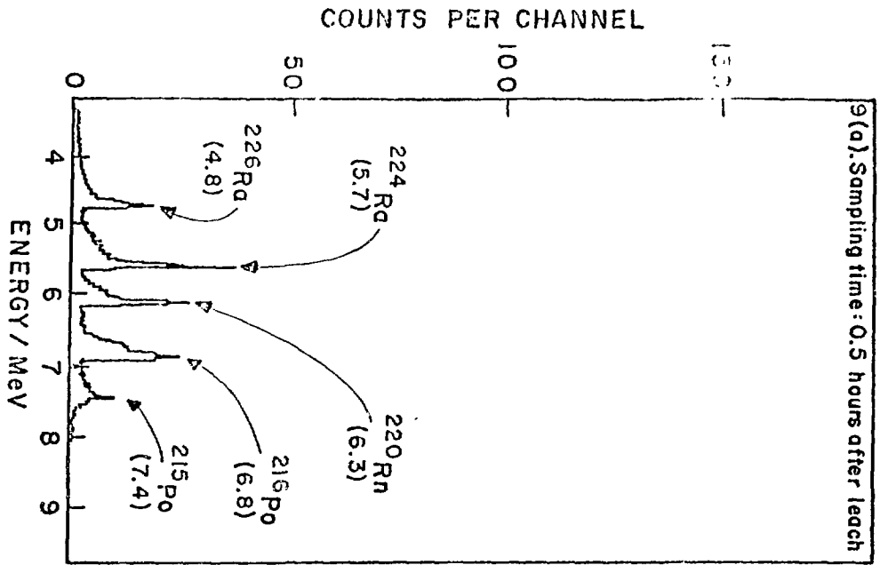
Figure 9. Spectra Obtained by Analysis of Fresh Liquors from Nitric Acid Leach. (Count Times = 2000s).
