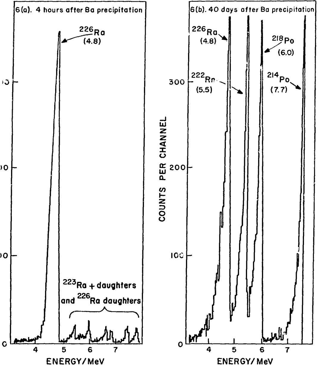
Figure 6. Spectra Obtained by Analysis of Old Residue from Nitric Acid Leach. (Count Times = 2000 s).
