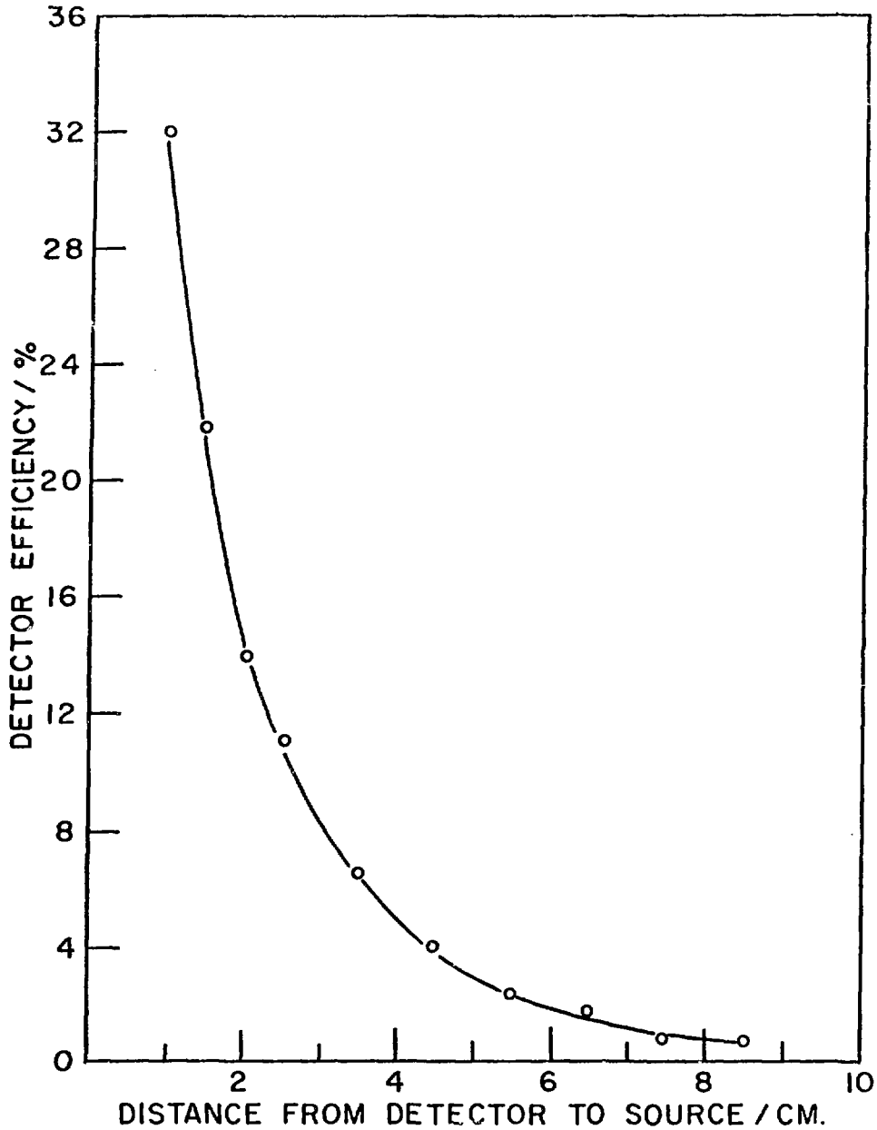
Figure 2. Variation of Detector Efficiency with Source-to-Detector Distance.
