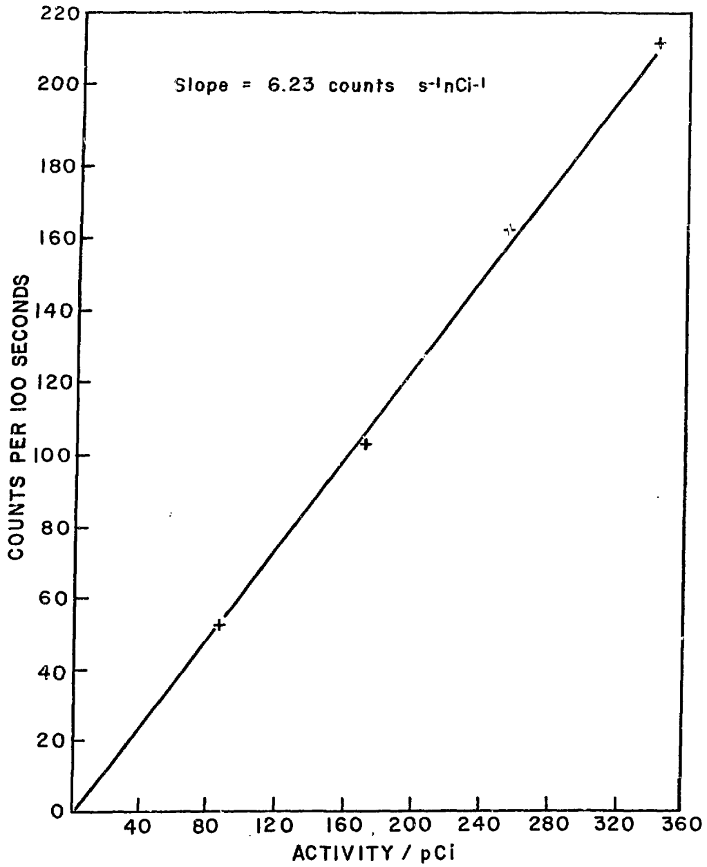
Figure 5. Calibration Curve for Alpha Activity.
