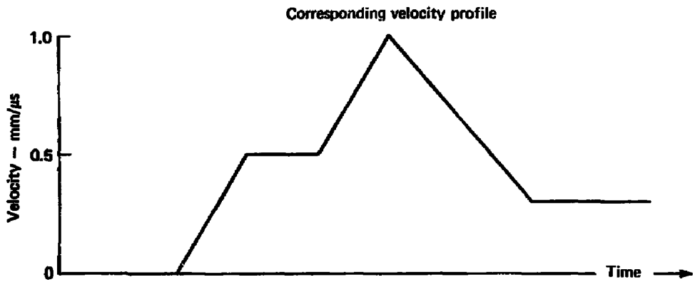
Fig. 2. Conversion of a fringe motion pattern to a velocity plot.
