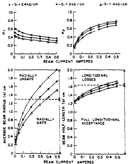
Fig. 5 Matched Beam Parameters as a Function of 750 keV Deuteron Beam Current
