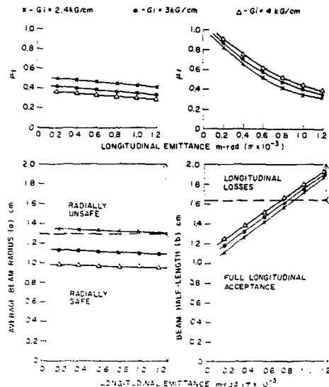
Fig. 7 Matched Beam Parameters as a Function of Longitudinal Emittance for a 750 keV Deuteron Beam Current of 0.2 Amperes.
