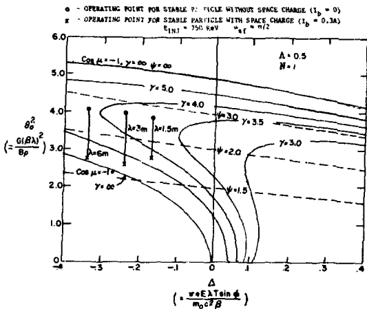
Fig. 1 Radial Stability Diagram
