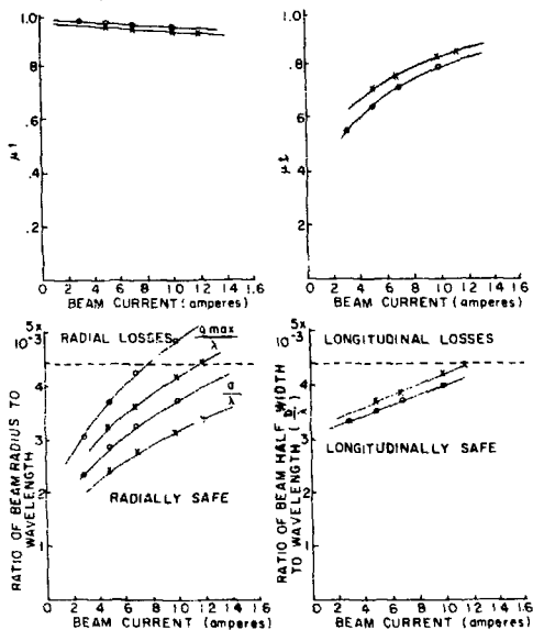
Fig. 6 Matched Beam Parameters as a Function of 750 keV Proton Beam Current
