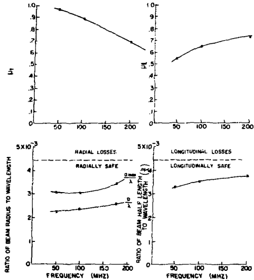
Fig. 4 Matched Beam Parameters as a Function of Frequency for a Proton Beam Current of 0.3 Amperes
