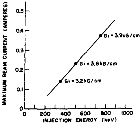
Fig. 3 Matched Beam Parameters as a Function of Injection Energy
