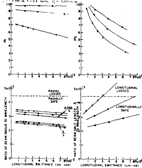
Fig. 9 Matched Beam Parameters as a Function of Longitudinal Emittance for a 750 keV Proton Beam Current of 0.3 Amperes
