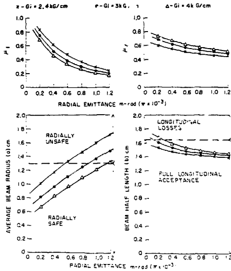
Fig. 8 Matched Beam Parameters as a Function of Radial Emittance for a 750 keV Deuteron Beam Current of 0.2 Amperes
