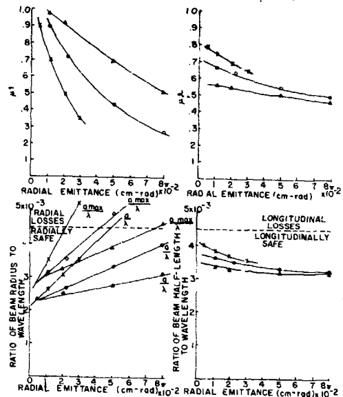
Fig. 10 Matched Beam Parameters as a Function of Radial Emittance for a 750 keV Proton Beam Current of 0.3 Amperes
