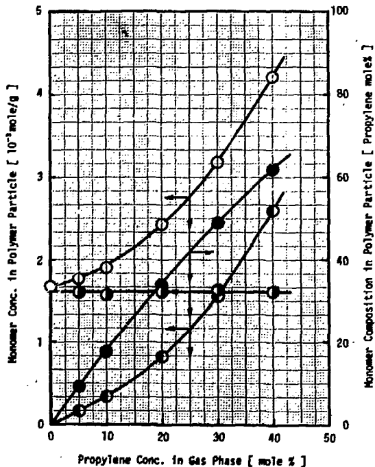
Fig.10. Relation between calculated monomer concentration in polymer particle and monomer composition in gas phase: (○), tetrafluoroethylene + propylene; (◐), tetrafluoroethylene; (●), propylene; (◑), propylene fraction of monomer in polymer particle; Pressure, 30 Kg/cm 2 G; temperature, 40 °C.
