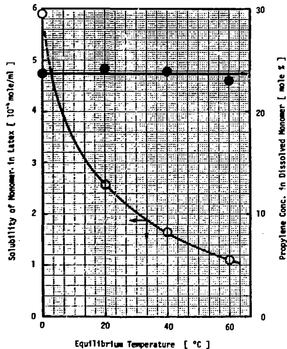
Fig. 9. Effect of temperature on solubility of monomer in latex: Pressure, 15 Kg/cm 2 G, propylene concentration in gas phase, 12.5 - 14.2 mole%; polymer concentration in latex, 16.8 wt%.
