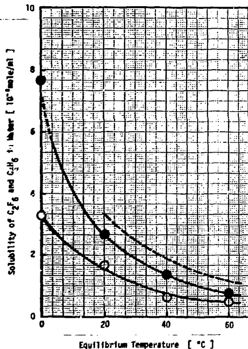
Fig. 3. Effect of temperature on solubility of tetrafluoroethylene (○) and propylene (●): Pressure of tetrafluoroethylene, 10 Kg/cm 2 G; pressure of propylene, 5 Kg/cm 2 G; (-----), solubility of propylene obtained by McKetta et al. at the pressure of 80 pisa.
