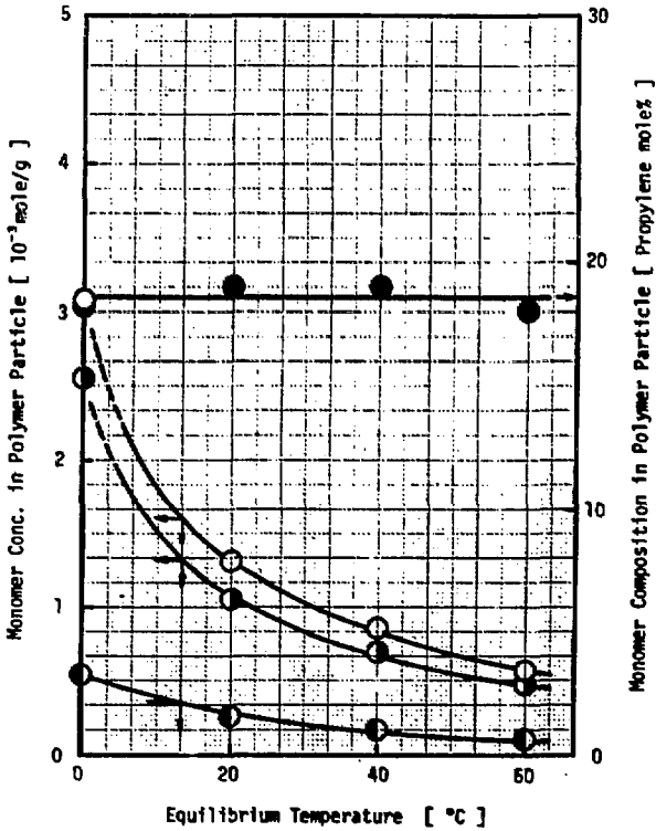
Fig.12. Relation between calculated monomer concentration in polymer particle and temperature: Pressure, 15 Kg/cm 2 G; propylene concentration in gas phase, 10 mole%; notations are same as Fig.10.
