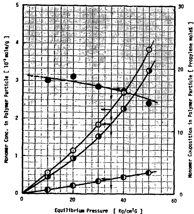
Fig.11. Relation between calculated monomer concentration in polymer particle and pressure: Temperature, 40 °C; propylene concentration in gas phase, 10 mole%; notations are same as Fig.10.
