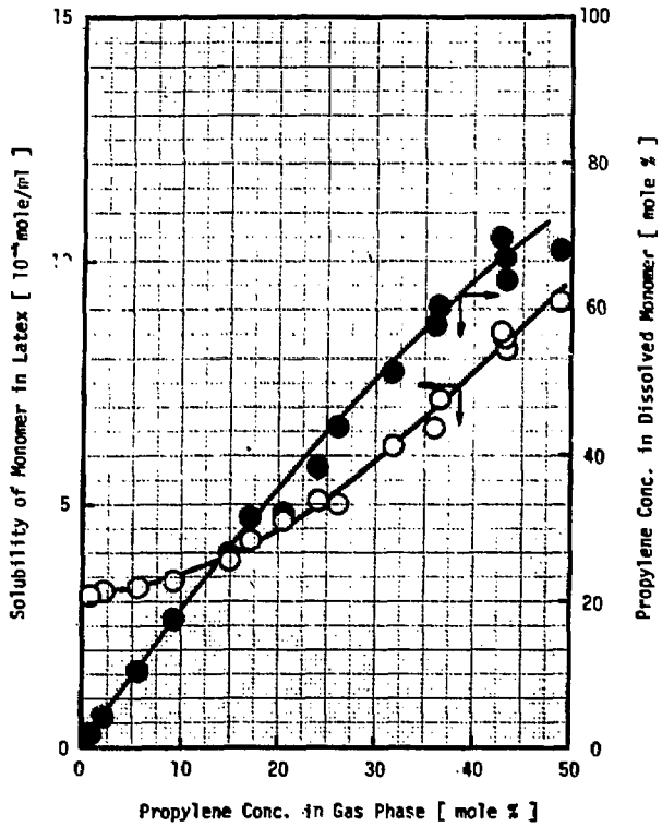
Fig. 7. Effect of monomer composition in gas phase on solubility of monomer in latex: Pressure, 30\text{Kg/cm}^2\text{G} ; temperature, 40^\circ\text{C} ; polymer concentration in latex, 16.8 wt%.
