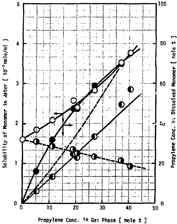
Fig. 4. Effect of monomer composition on solubility of monomer in water: (O), solubility of monomer mixture of tetrafluoroethylene and propylene; (◐), solubility of tetrafluoroethylene; (◑), solubility of propylene; (●), propylene concentration in dissolved monomer; (-----), calculated solubilities of tetrafluoroethylene and propylene with the data shown in Fig.2; pressure, 30 \text{ Kg/cm}^2\text{G} ; temperature, 40 \text{ }^\circ\text{C} .
