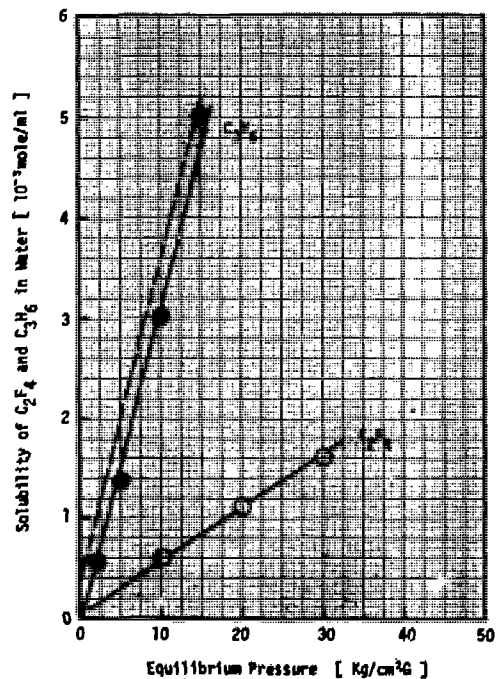
Fig. 2. Effect of pressure on solubility of tetrafluoroethylene (○) and propylene (●): Temperature, 40 °C; (-----), solubility of propylene obtained by McKetta et al. at the temperature of 100 °F.
