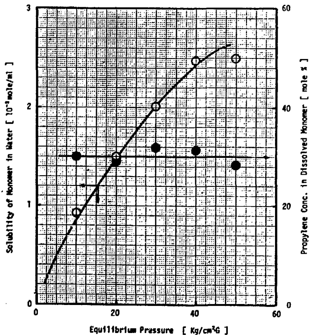
Fig. 5. Effect of pressure on solubility of monomer in water: Temperature, 40 °C; propylene concentration in gas phase, 9.2 - 11.8 mole%.
