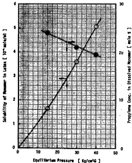
Fig. 8. Effect of pressure on solubility of monomer in latex: Temperature, 40 °C; propylene concentration in gas phase, 11.5 - 12.5 mole%; polymer concentration in latex, 16.8 wt%.
