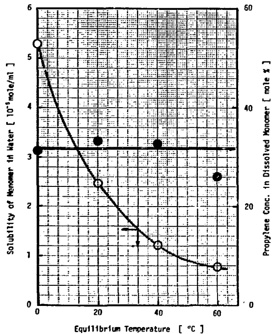
Fig. 6. Effect of temperature on solubility of monomer in water: Pressure, 30 Kg/cm 2 G; propylene concentration in gas phase, ca. 11.5 mole%.
