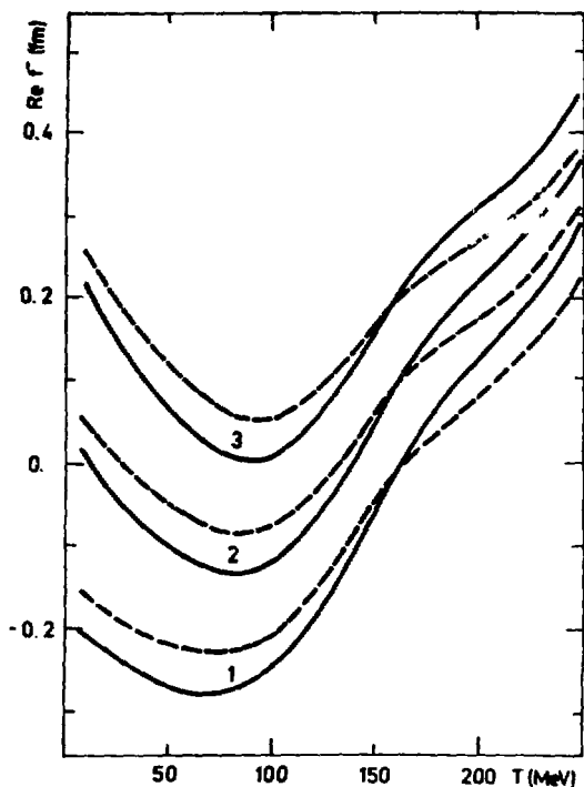
Fig.4. The real part of the antisymmetric scattering amplitude as a function of the kinetic laboratory energy for f_{\pi}^2 \text{ } ^3\text{He} \text{ } ^3\text{H} = 0., 0.08 and 0.16 - curves 1,2 and 3, respectively, with (solid lines) and without (broken lines) Coulomb corrections.
