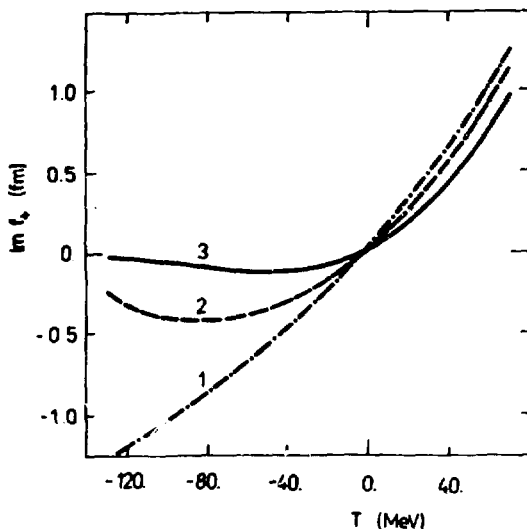
Fig. 2. The imaginary part of the forward \pi^+ \text{He}^3 scattering amplitude in the physical region from the extrapolation of eq.(4) with n=0,1 and 3 - curves 1,2 and 3, respectively.
