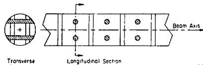
Fig. 3. Section of jungle-gym structure.
