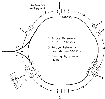
Fig. 1. PEP RF Reference Line layout.
