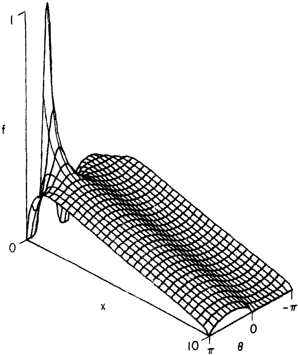
Fig. 2. Surface of f(\theta, x) using the boundary data given in Fig. 1.
