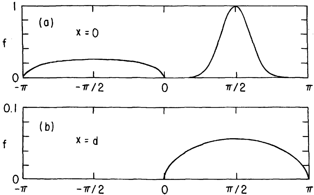
796032 Fig. 1. Data on the boundaries. (a) f(\theta) vs. \theta on the boundary at x=0 ; for \theta > 0 , the data is given, whereas for \theta < 0 the data is computed, using 250 eigenfunctions. (b) f(\theta) vs. \theta on the boundary at x=d ; \theta < 0 , the data is given, whereas for \theta > 0 the data is computed. Note change of scale.
