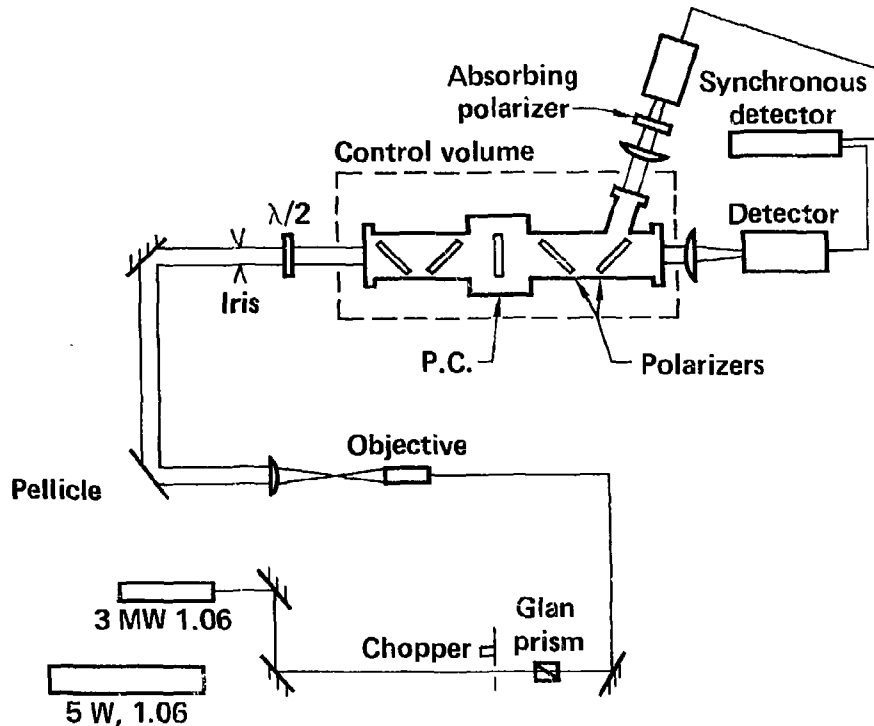
02-01-1279-5176 Fig. 2 - Experimental Layout: A chopped cw 1.06 μm beam is expanded, polarized and passed through the Pockels cell polarizer assembly, which is in a chamber maintained at a controlled temperature and humidity. The reflected and transmitted beams are collected, synchronously detected, and ratioed.
