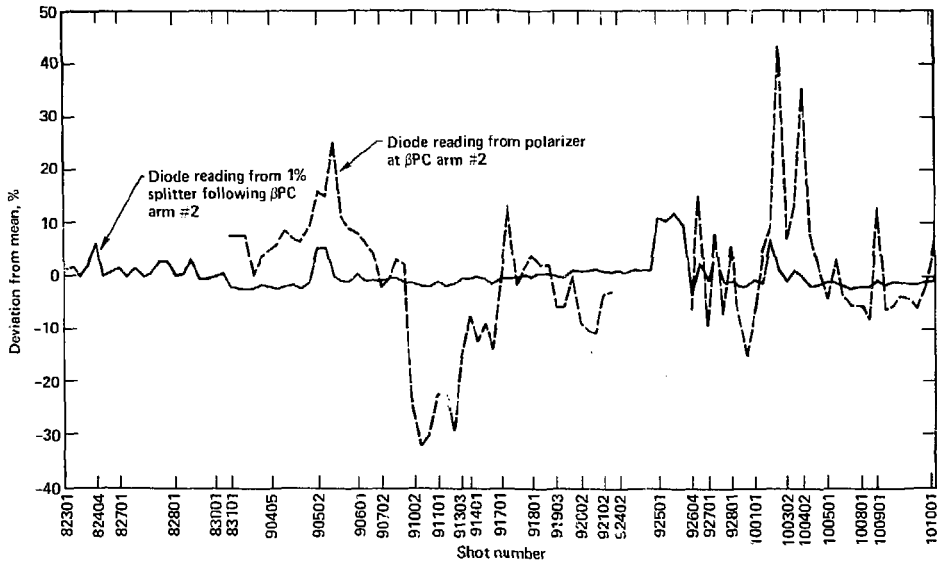
02-90-1079-4544 Fig. 6 - Prototype Beamsplitter Stability: Calibration of a prototype beamsplitter installed at the Pockels cell polarizer assembly output has remained stable. The detector on the polarizer underwent large fluctuations during the same test period.
