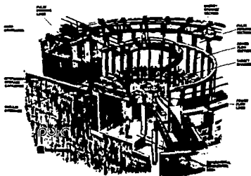
Fig. 4. PFBA-I Artist's Conception.
