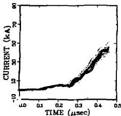
Fig. 14. Mark Generator Timing Data.
