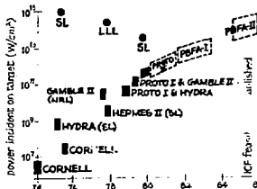
Fig. 1. Light Ion Beam ICF.
