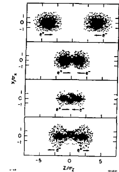
Fig. 4--Side view of the collision of oppositely charged beams, showing the pinch effect for Gaussian profiles and a disruption factor D = 14.4 .
