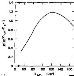
Fig. 6--Initial design luminosity vs center-of-mass energy.
