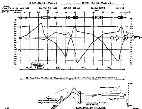
Fig. 8--Schematic representation of the final focusing system.
