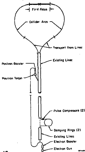
Fig. 1--General layout of the single pass collider.
