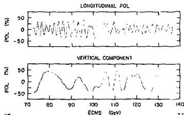
Fig. 10--A model calculation of spin projections in the interaction region as a function of center-of-mass energy, for 50% polarization leaving the linac. The g-2 precession of the electron spin results in rapid oscillations of the longitudinal component and rather slower oscillations of the vertical component from a beam-transport system that approximates the north arc of the Collider ring.
