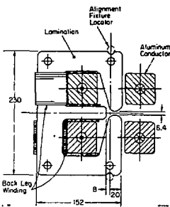
Fig. 7--Cross section of the SLC arc magnets. Dimensions are in millimeters.
