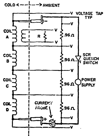
Fig. 5 Electric Diagram of Coil Tested With Secondary in Shell Coil "A" Only.
