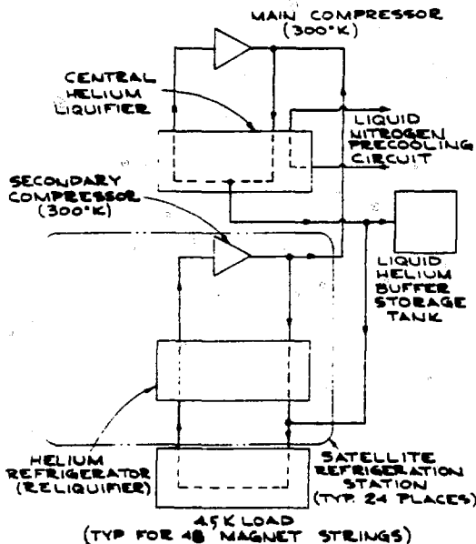
Fig. 2. Doubler Cryogenic System block diagram.
