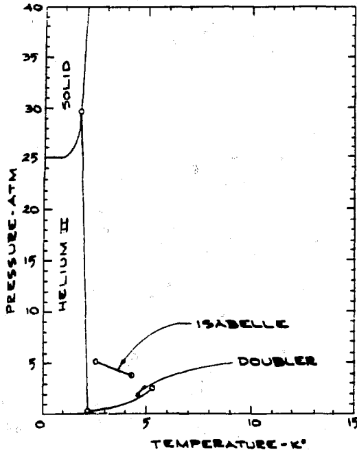
Fig. 3. System Operating Points
