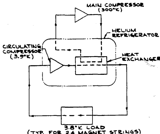
Fig. 1. ISABELLE Cryogenic System block diagram.
