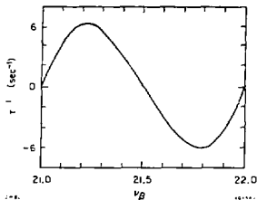
Fig. 2. Instability growth rate (damping rate if negative) versus the unperturbed betatron tune for the rigid bunch mode m = 0 with a 14.5 GeV, 1 ma single-bunch beam. The radiation damping rate at 14.5 GeV is 110 \text{ sec}^{-1} .
