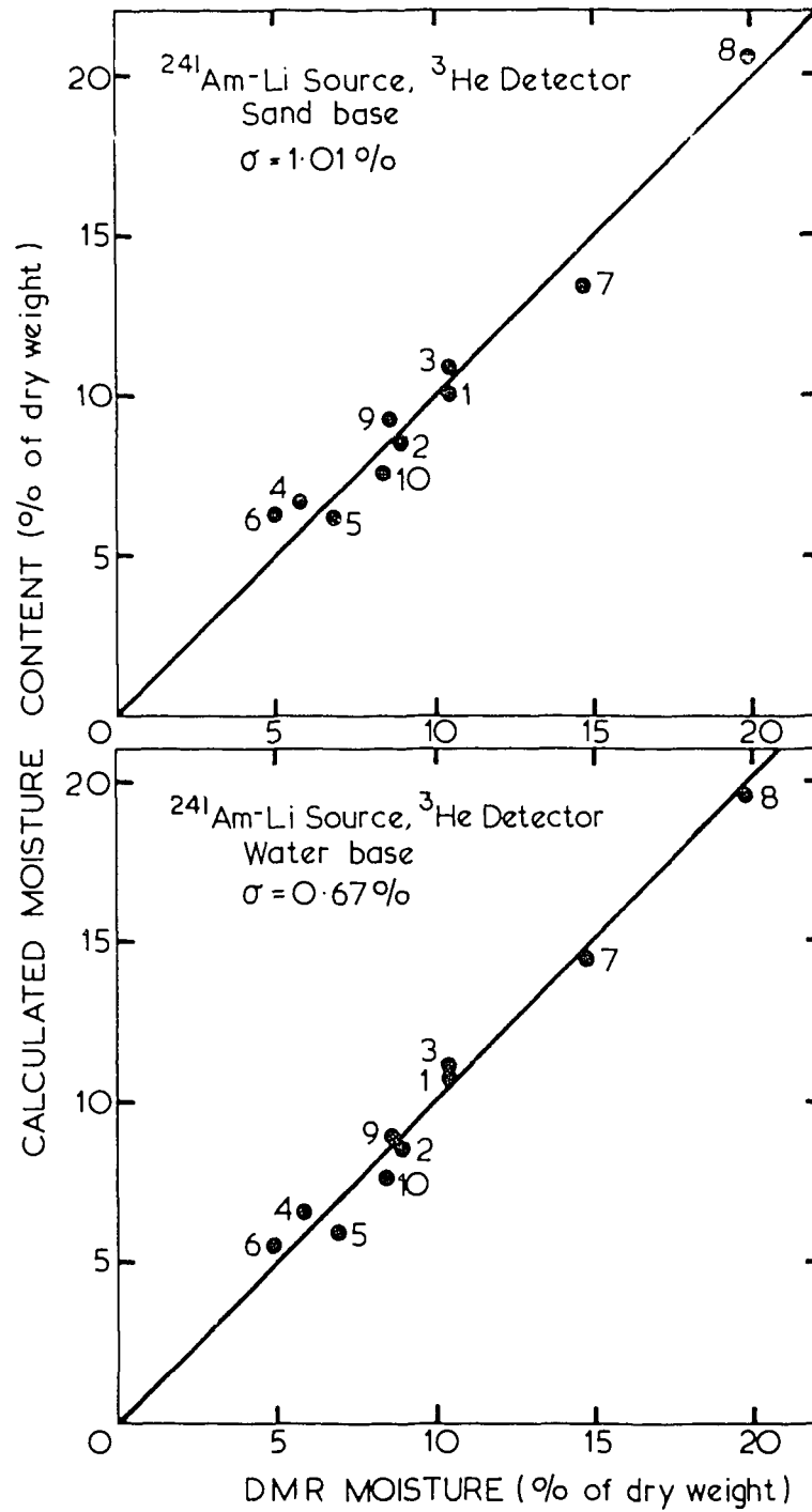
Figure 6. Calculated versus measured moisture contents for the probe containing the ^{241}\text{Am-Li} source and ^3\text{He} detector. The calculated moisture content was determined from the measured ^3\text{He} count rate and the wet bulk density value supplied by the DMR
