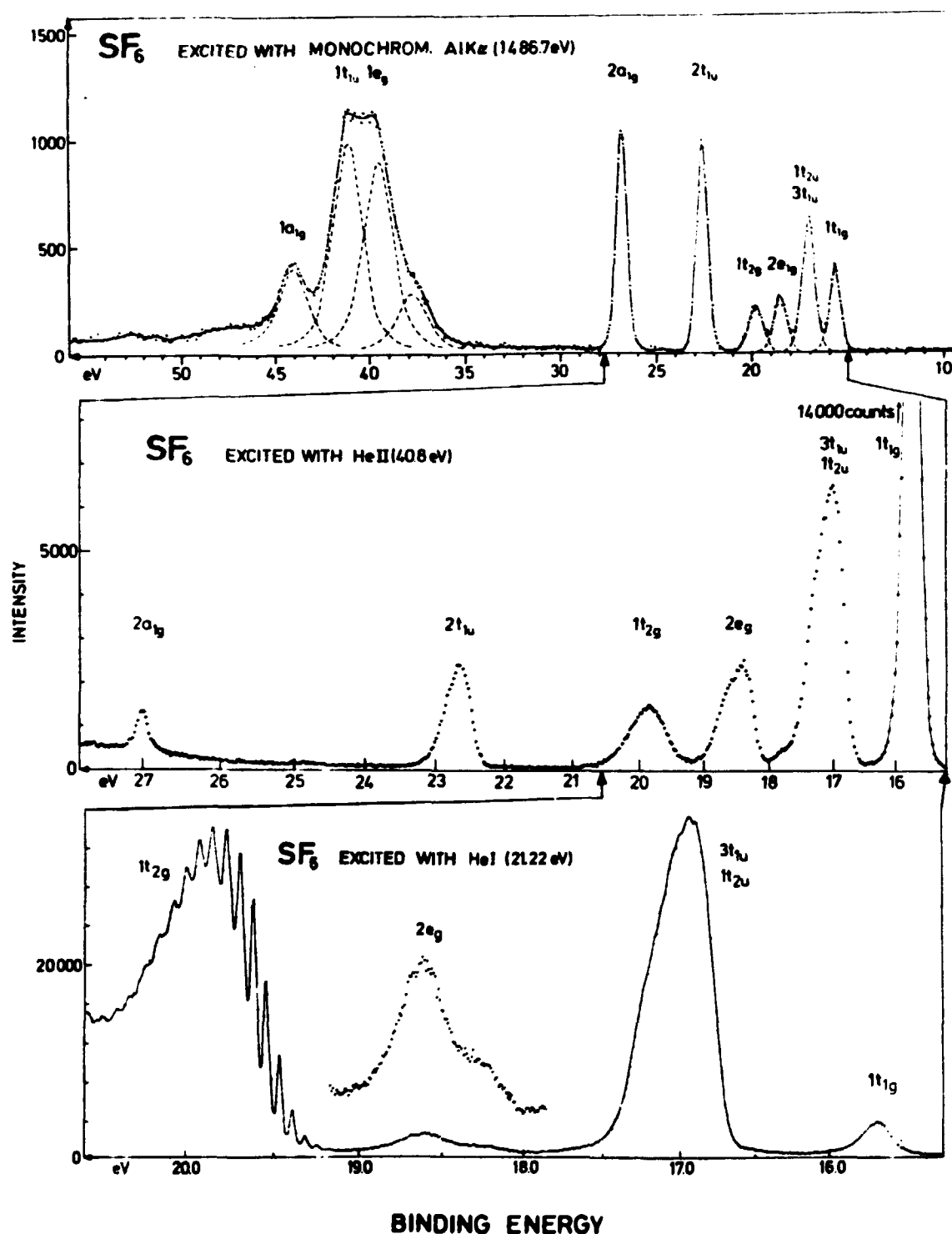
Fig.14. Valence electron spectra of the SF 6 molecule excited with different photon energies (AlK \alpha -, HeII and HeI-radiations). This figure illustrates the complementary nature of the various excitation sources. The AlK \alpha -excited spectrum enables a recording of the full valence region (including the innermost orbitals), which is not possible with the lower photon energies. The higher resolution in the spectra excited with the He resonance radiations allows the study of finer details of each of the outer electron bands. Note also the strong variations in the relative intensities of the bands as a function of photon energy. This can be used as an aid in assigning the spectrum /197,198/.
