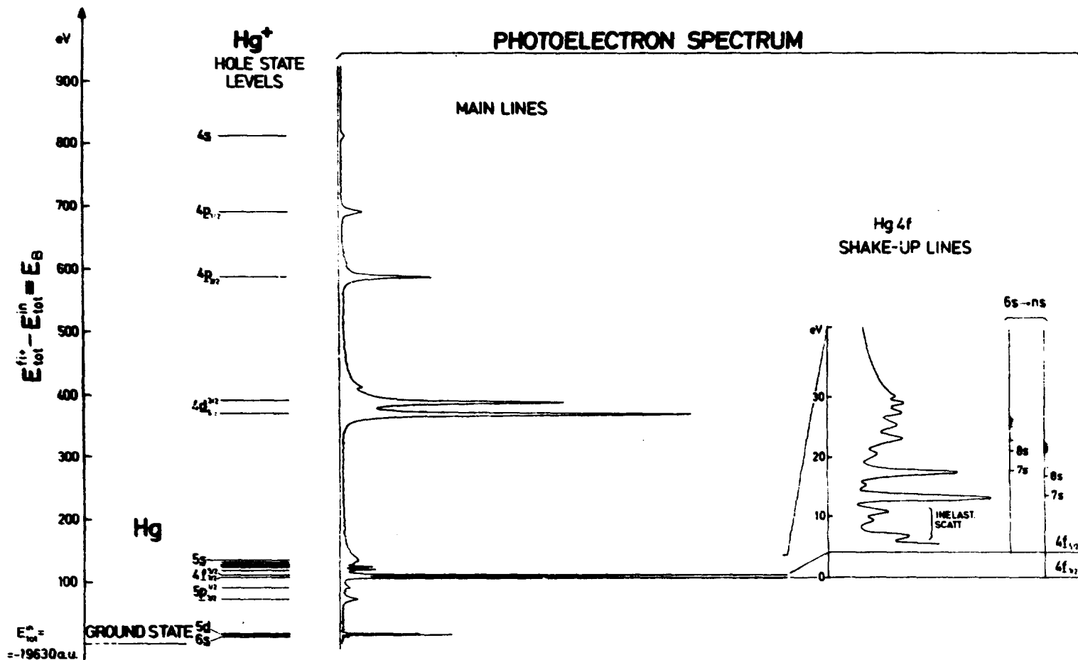
Fig. 8. Relation between the hole-state level system and observed photoelectron spectrum for the mercury atom. The figure illustrates that the main lines are connected with states of the ion where (in a one-electron picture) an atomic orbital has been removed from the neutral ground state. The energy region close to the 4f-lines has been expanded (far right) to show that the additional satellite lines observed (shake-up lines) are due to excitations ( 6s \rightarrow ns ) above the 4f hole ground states. (Note that the intensities of the 4f-lines have been truncated to fall into the scale of the figure.) (From refs. 114 and 260.)
