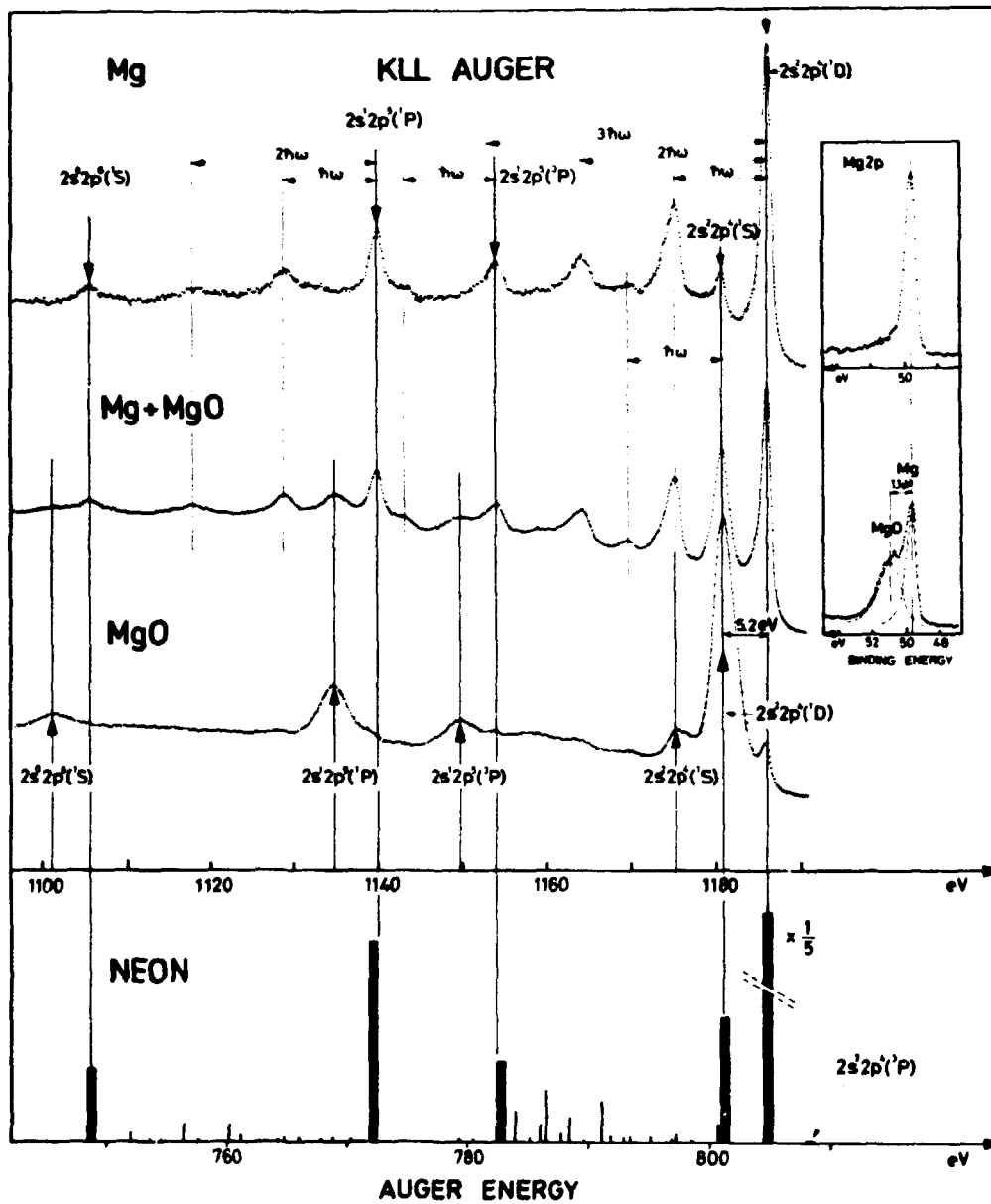
Fig.7. MgKLL Auger electron spectra at different stages of oxidation as obtained in ESCA. Upper spectrum is from a clean metal surface, lower spectrum from the oxidized metal (with only a trace of metal) and the middle spectrum is from an intermediate oxidation. Volume plasmon lines are observed. For comparison, the positions of the NeKLL Auger electron lines are given below, as recorded in the ESCA instrument by means of electron beam excitation.
