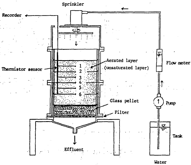
Fig.5 Measured point in soil layer model apparatus
