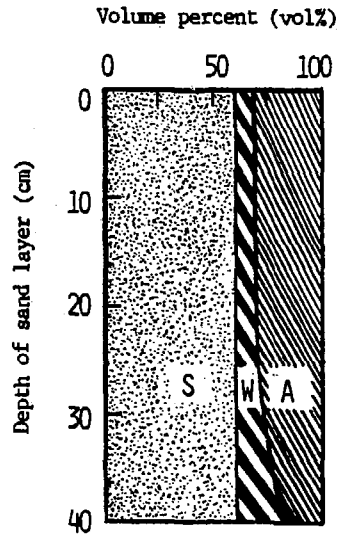
Fig.6 Three phase distribution curve W; Water retention ratio (vol%) S; Solid ratio (vol%) A; Porosity (vol%)
