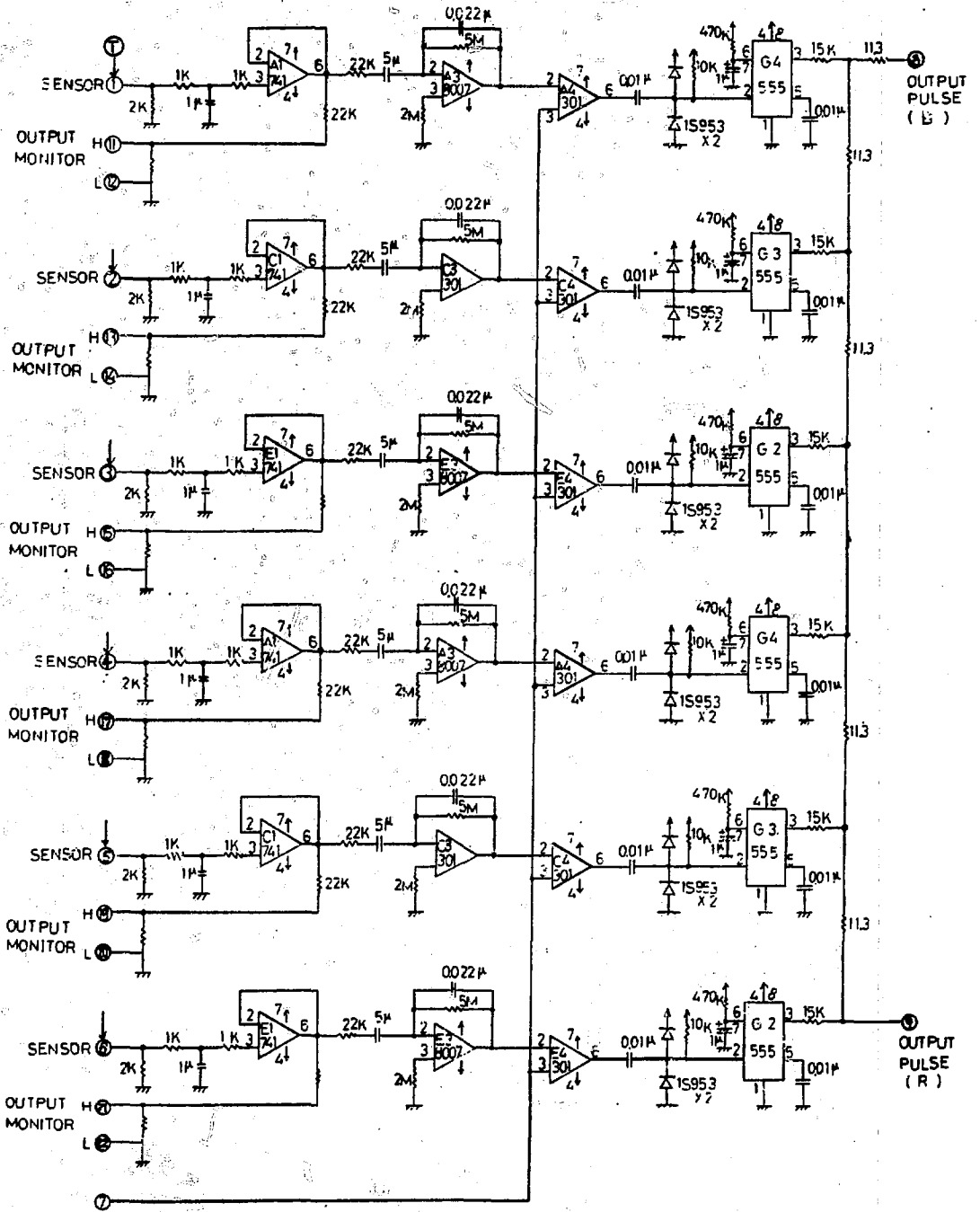
Fig.4 Electrical circuit for pulse converter
