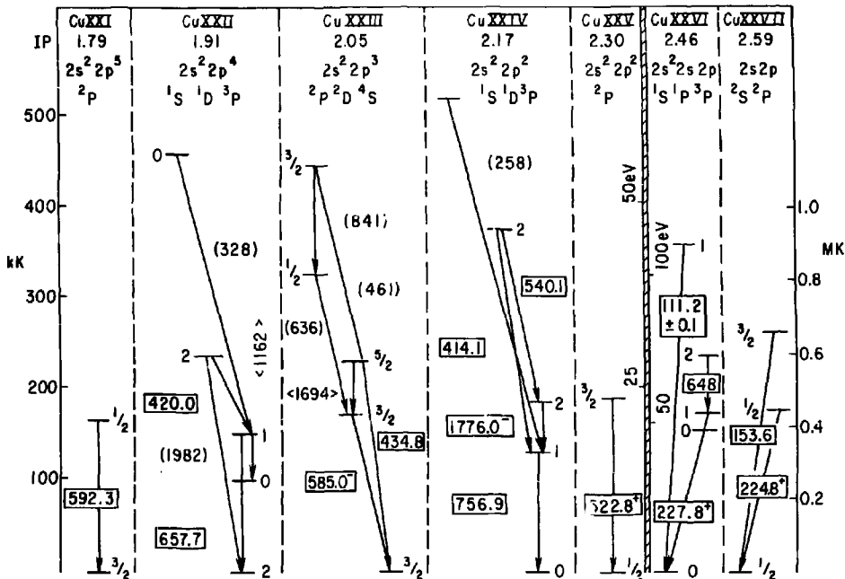
Fig. 3 The 2s^2 2p^x ground configurations and the 2s-2p , 2s^2-2s2p transitions in copper. Observed wavelengths in boxes. Ionization potentials indicate approximate temperature of maximum emissivity in tokamak discharges.
