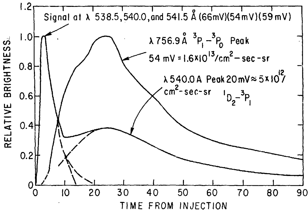
Fig. 2 Appearance of interfering radiation, ascribed to earlier states of ionization of copper, in the neighborhood of the \lambda 540.0 Å intercombination line of Cu XXIV, 2s^2 2p^2 configuration.
