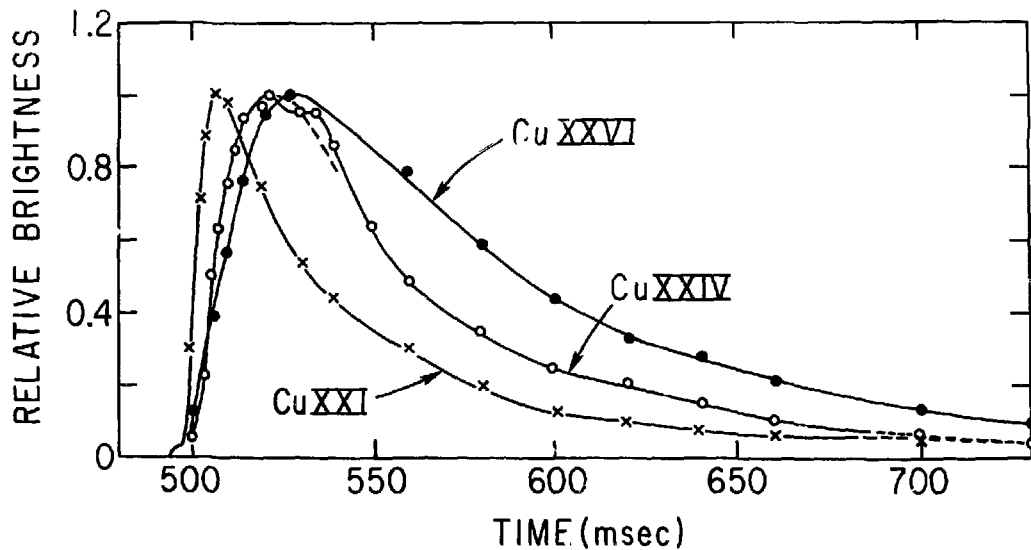
Fig. 1 Time behavior of observed brightness of three copper lines after injection (arrow): Cu XXI \lambda 592.3 Å, Cu XXIV \lambda 756.9 Å, and Cu XXVI \lambda 111.2 Å.
