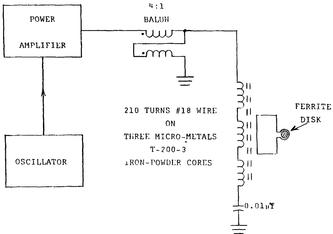
Figure 1. Schematic diagram of the ferrite modulator circuit.
