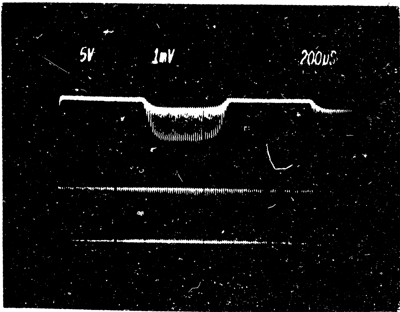
Figure 5. Nearly 100% modulation of a 0.307 \mu\text{m} wavelength laser has been achieved with a \text{LiTaO}_3 electro-optic crystal.
