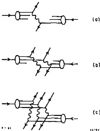
Fig. 7. QCD contributions to high p_T processes. The multiparticle 2+2 and 3+3 reactions produce high transverse energy events with a large fraction of the available energy. More complicated reactions with gluons and sea quarks are not shown.
