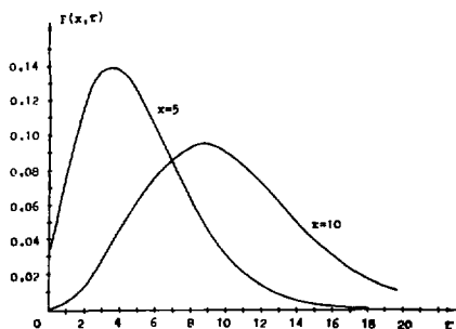
Fig. 1. Probability distribution of time delay at the stage of compound nucleus calculated by formula (20) ( x = \frac{2\pi\Gamma}{nD} , \tau = \frac{\hbar}{\Gamma} ).
