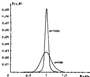
Fig. 2. Plot of the probability distribution of time delay at a very large density of resonances levels ( x = \frac{2\pi\Gamma}{nD} , \tau = \frac{\hbar}{\Gamma} ).
