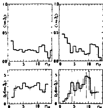
Fig.2. Dependences of the average values \langle\cos\theta_p\rangle , where \theta_p is the proton emission angle, on the proton multiplicity in pion-xenon nucleus collisions without particle production at 3.5 GeV/c momentum - upper; n_p - dependences of the normalized dispersion D/\langle\cos\theta_p\rangle - lower. Left - in the sample of events of the type (1a) and (1b) together, right - in the sample of events of the type (1a).
