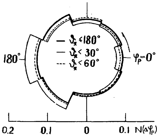
Fig.12. Distributions N(\Delta\phi_p) of the azimuth angles \phi_p of the emitted protons in pion-xenon nucleus collision events at 3.5 GeV/c momentum in which particle production does not occur, in classes of events of the type (1b) with various deflection angles \theta_{\pi} of the incident pion. The proton emission azimuth angle \phi_p is defined as the angle between the point deflection plane and the proton emission plane.
