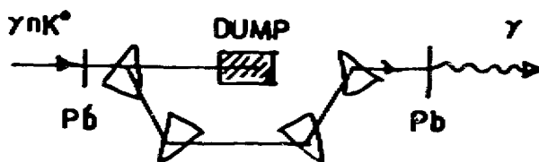
Fig. 3. Photon beams by synchrotron radiation separation, hadronic filtering, and \gamma = e^- \rightarrow \gamma conversion.
