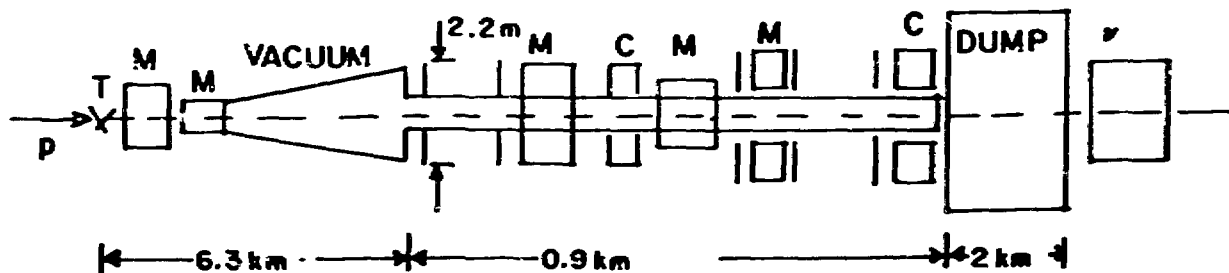
Fig. 2. Tagged \nu beam from K^0 \rightarrow \pi \nu, \tau \nu . T is the target, M's are magnets, C's are e.m. and hadronic calorimeters for evt identification.
