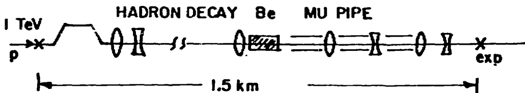
Fig. 1. Tevatron II muon beam design (Ref. 8).
