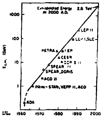
Fig. 2. Growth of electron colliders.
