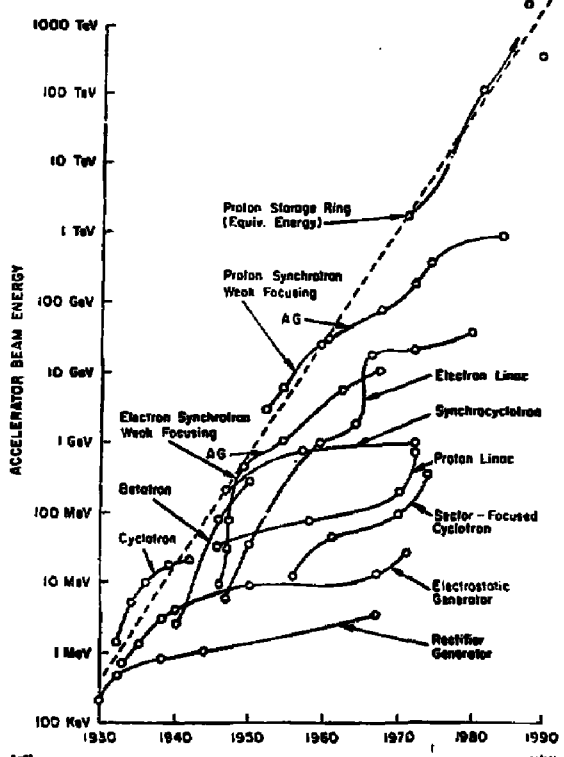
Fig. 1. Energy growth of accelerators and storage rings.
