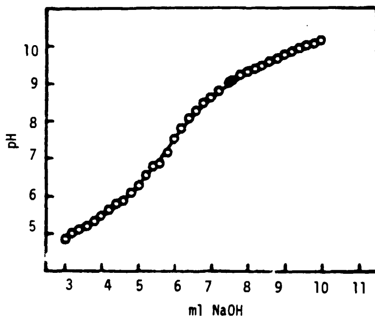
Figure 3. A titration curve of 0.040 g Lake Bradford humic acid by 0.02 M NaOH at a constant ionic strength of 0.1 M (8).
