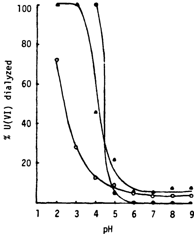
Figure 10. Dialysis of an aqueous solution of U(VI) in 0.01 M \text{KNO}_3 as a function of pH (15).
