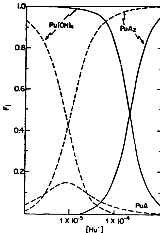
Figure 9. Calculated fractional ( F_i ) concentration of a hypothetical plutonium(IV) humate complex as a function of the humate concentration at pH 5.5 (---) and 7.5 (—) (12).
