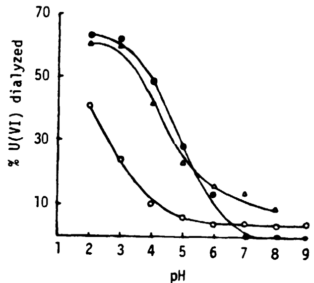
Figure 11. Dialysis of an aqueous solution of U(IV) in 0.01 M \text{NaCl} as a function of pH (15).
