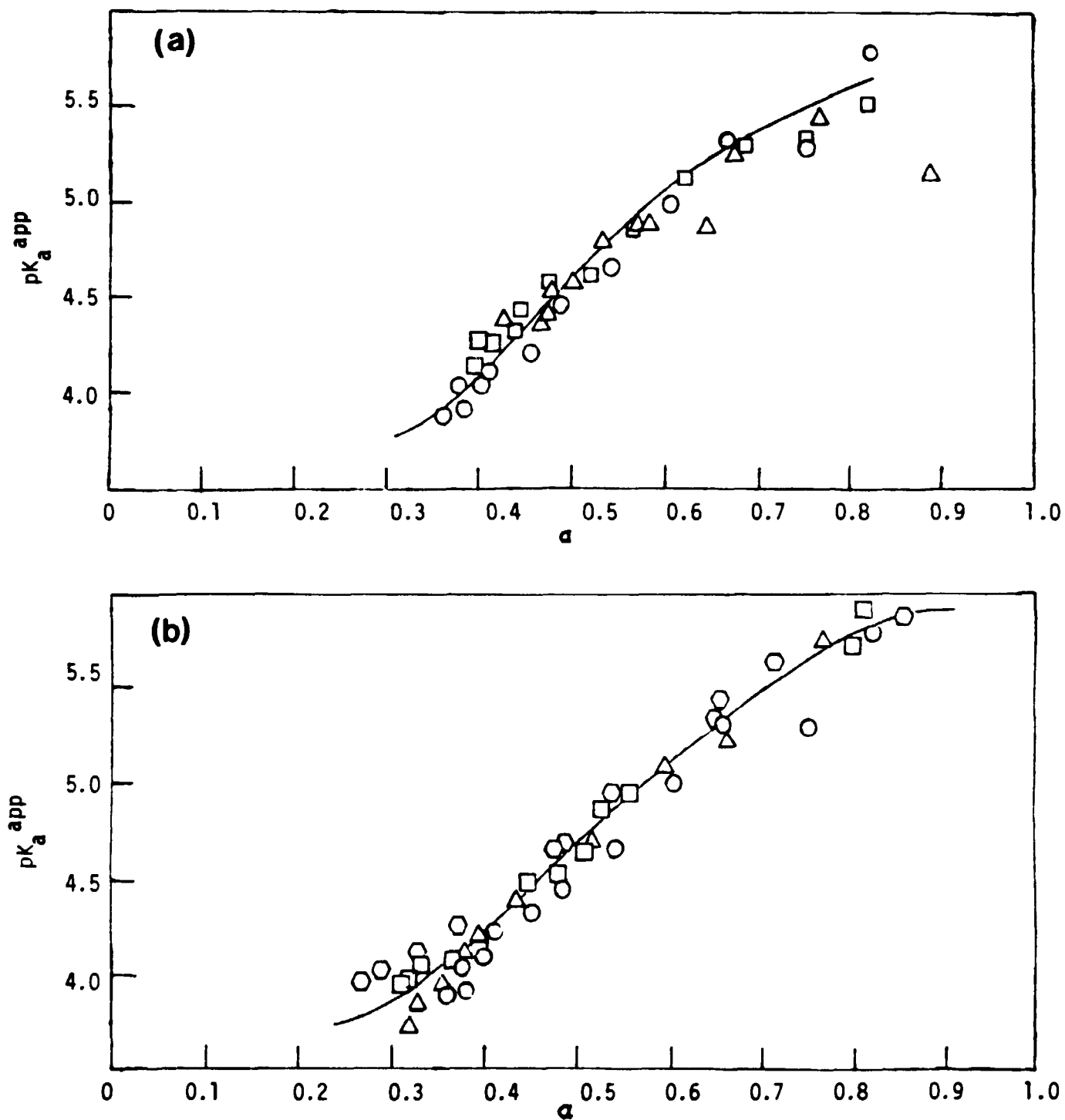
Figure 6. Plots of the apparant pK_a -values as a function of the degree of dissociation, \alpha , for Armadale fulvic acid (2) (a) \circ 1.3 \times 10^{-4} g/ml; \square 6.0 \times 10^{-5} g/ml; \triangle 3.0 \times 10^{-5} g/ml; initial capacity ( 6.7 \pm .3 meq/g) and ionic strength (0.1 M NaCl) kept essentially constant. (b) \circ 0.10 M NaCl; \square 0.030 M NaCl; \triangle 0.010 M NaCl; \odot 0.0050 M NaCl; initial capacity ( 7.1 \pm 0.5 meq/g) and initial concentration ( 1.2 \pm 0.08 \times 10^{-3} M) kept essentially constant.
