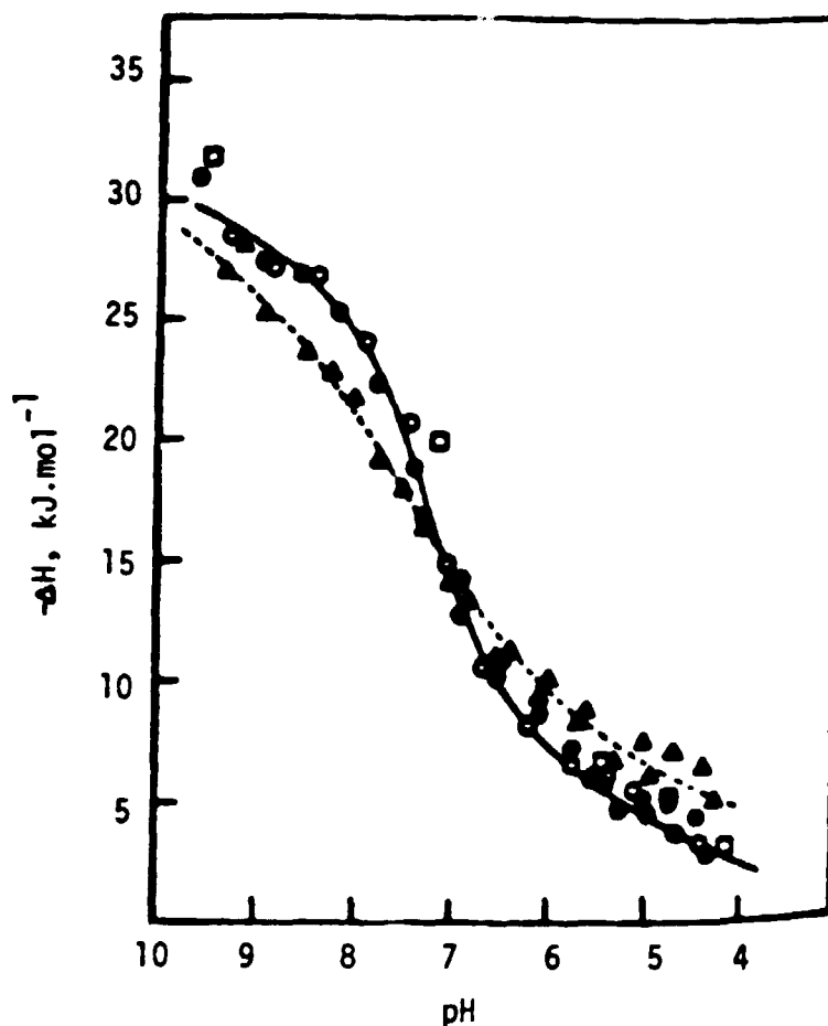
Figure 5. Variation of the enthalpy of protonation as a function of the pH of the measurement (8).
