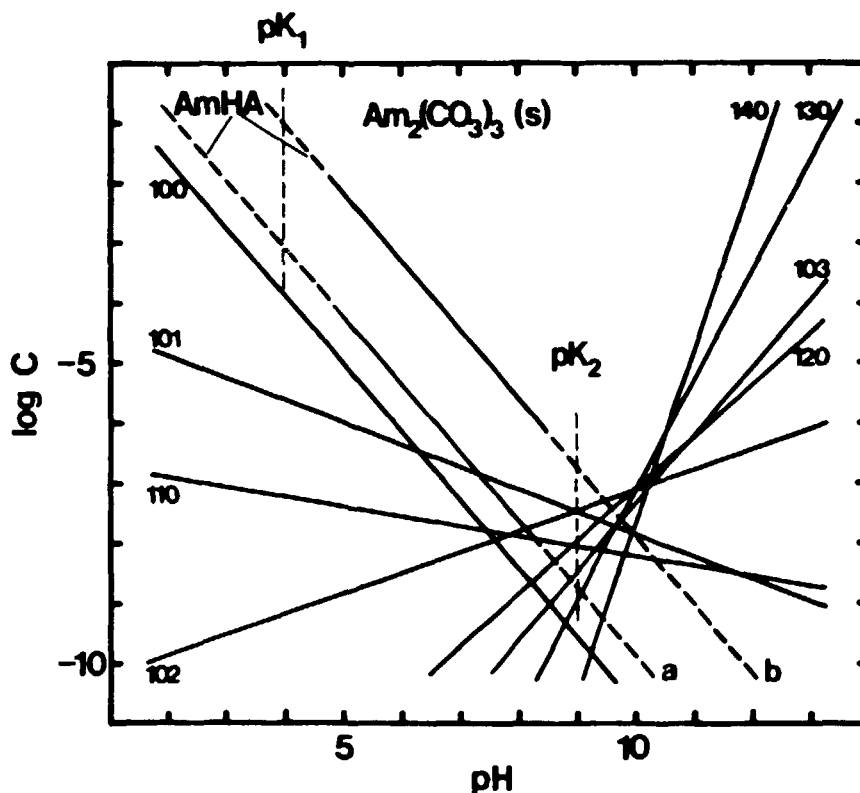
Figure 1-2. Speciation in a \text{Am}^{3+} - \text{OH}^- - \text{CO}_3^{2-} -HA-system a. 0.1 mg/l HA b. 10 mg/l HA
