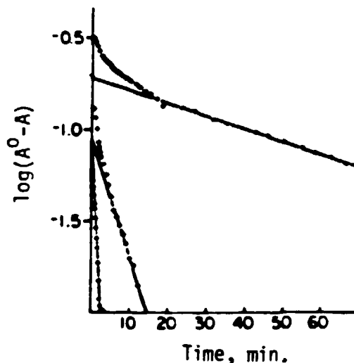
Figure 13. Resolution of the observed curve of the dissociation of thorium-humate with time. [ThH\bar{U}] = 5.77 \times 10^{-6} M, [H\bar{U}] = 1.20 \times 10^{-4} M, [xy1. Or] = 9.85 \times 10^{-5} M, [Ac_T] = 0.01 M, pH = 4.33 (18).
