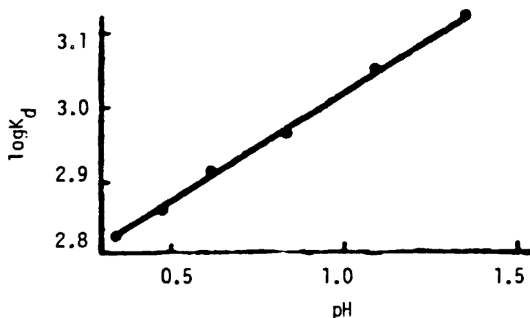
Figure 12. The sorption of plutonium by humus substances as a function of pH (10).
