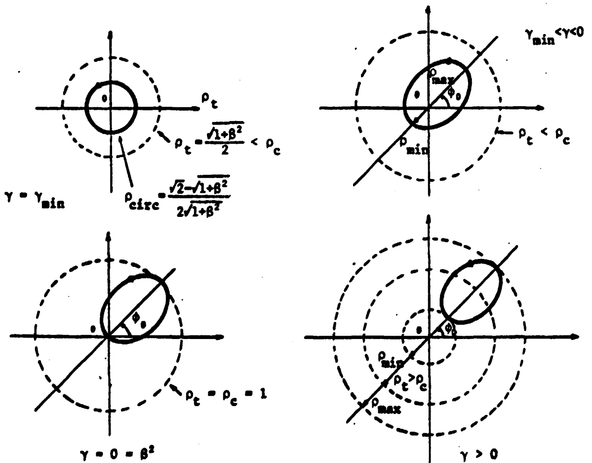
FIGURE 4: Graphs of the trajectories in the (\rho, \phi) -plane for several values of \gamma , with respect to \rho_c (Gödel's critical radius \rho_c = \sinh^2 r = 1 ) and \rho_t (for values of \rho beyond \rho_t the time-coordinate t decreases).
