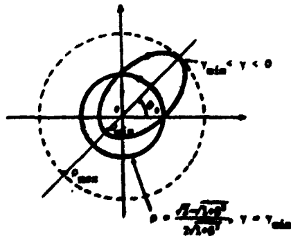
Fig. 2b: \gamma < 0
