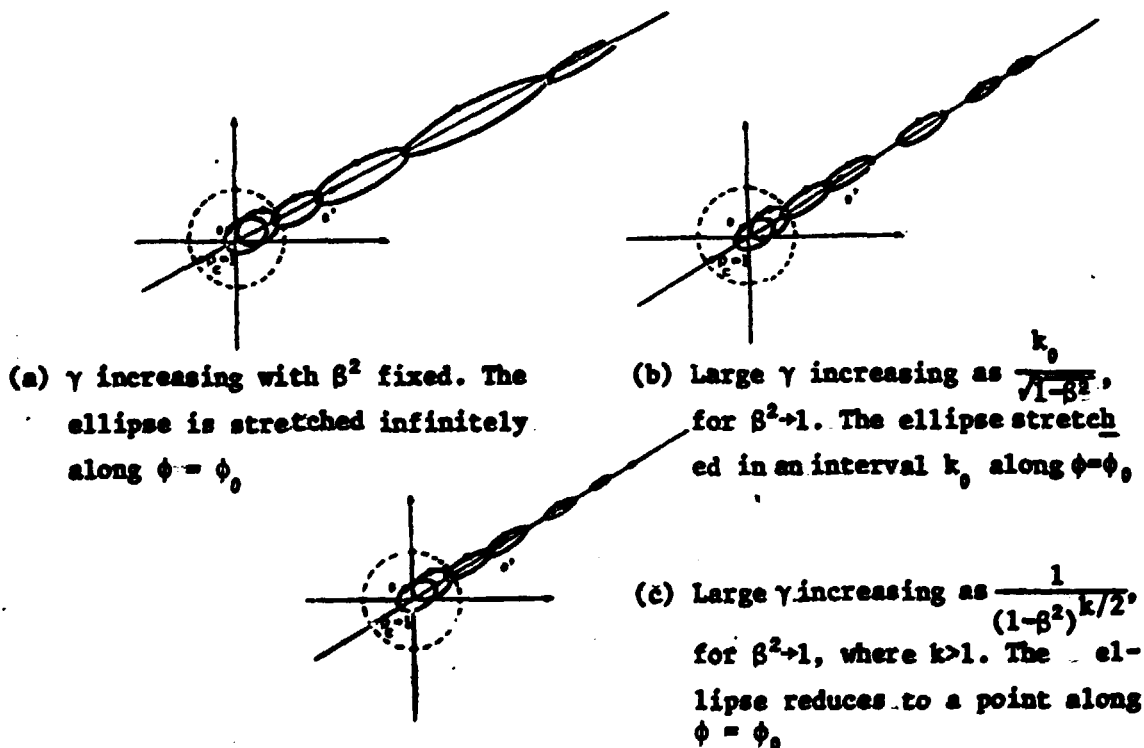
FIGURE 3: Graphs of the (\rho, \phi) -trajectories for increasing \gamma
