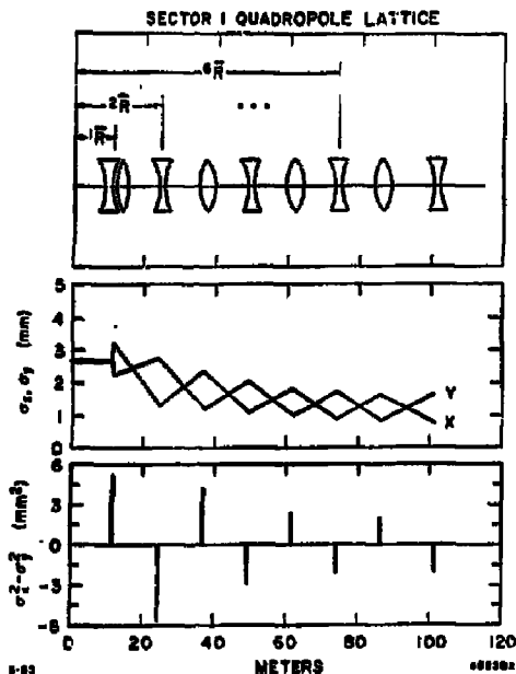
Fig. 4. (a) Quadrupole lattices in first 100 meters of the line; (b) \sigma_x and \sigma_y versus x ; (c) \sigma_x^2 - \sigma_y^2 versus x .
