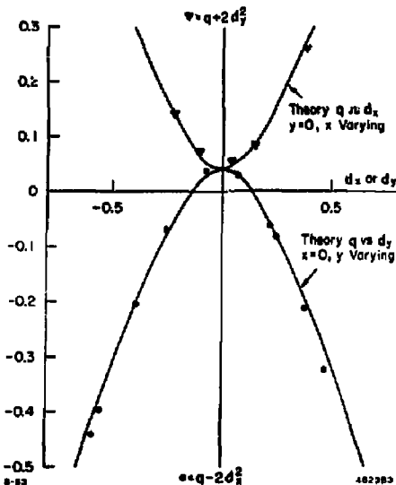
Fig. 3. Monitor Sensitivity. q + 2d_x^2 versus d_x (triangles). q - 2d_y^2 versus d_y (circles). Vertical intercept = 2(\sigma_x^2 - \sigma_y^2/a^2) .
