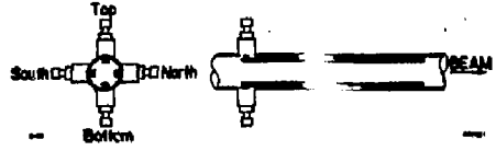
Fig. 1. Stripline position monitor.
