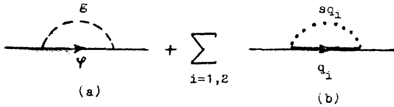
Fig. 3. Gluino wave function renormalization in one-loop approximation. We denote the quark field by q_i where i is the flavor index; the corresponding scalar quark is denoted by sq_i .
