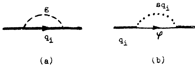
Fig. 4. Quark wave function renormalization in the same approximation.
