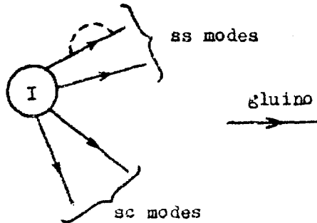
Fig. 1. Instanton-induced effective interaction in the simplest SYM theory ( n = 1, N = 2 ). Dashed line shows the external line renormalization which is included in eqs. (5), (9) and others of that type. Proper vertex corrections are absent (sect. 3).
