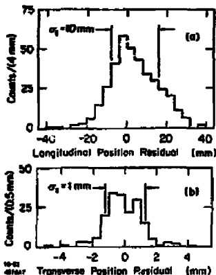
Fig. 7. Residual distribution in the PSC coordinates. a) Longitudinal coordinate derived from the time difference in the strip ends. b) Transverse coordinate calculated as the charge weighted centroid taken over all the strips. The particles were tracked by a drift chamber telescope.
