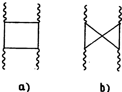
Fig.2. Pauli principle corrections K^J into the traditional QPM equations 1/ corresponding to the well-know secular equation:
