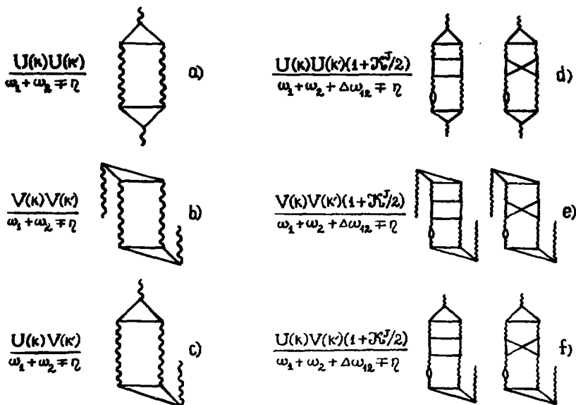
Fig.3. Correspondence between the diagrams included in the QPM with the matrix elements M_{kk'} (12) a,b,c) if the corrections of the Pauli principle are neglected. d,e,f) if the corrections of the Pauli principle are taken into account.
