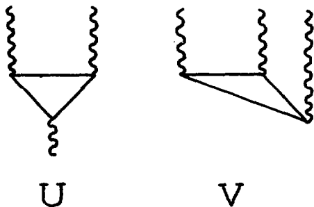
Fig.1. The vertices U and V.
