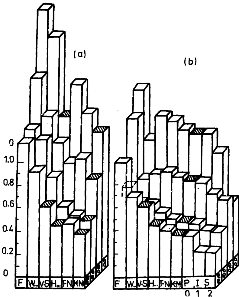
Fig.6. The standard deviation of various formulae in each group of nuclei for both old (a) and new (b) values of the additive parameters.
