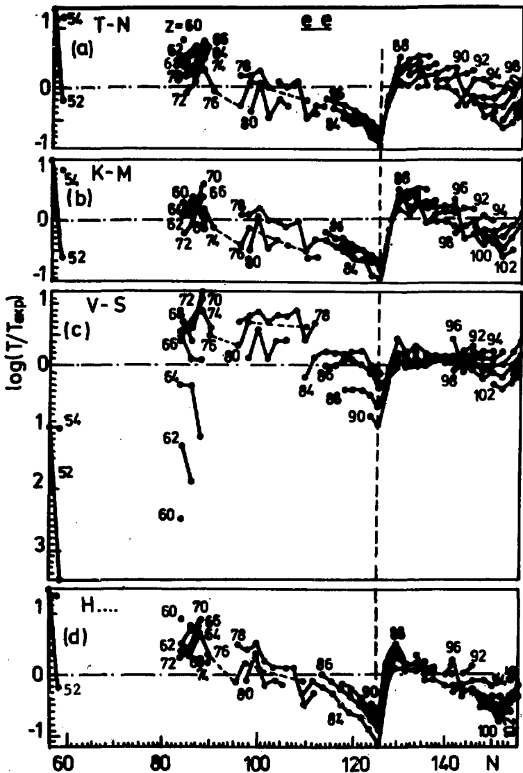
Fig.2. The errors of life-time predictions with Taagepera-Nurmis's (a), Keller-Minzel's (b), Viola-Seaborg's (c) and Hornshøj's et al. (d) formula for even-even nuclei.
