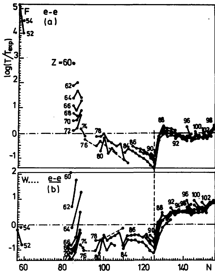
Fig.1. The error of life-time predictions with Fröman's (a) and Wapstra's et al. (b) formula for even-even nuclei.
