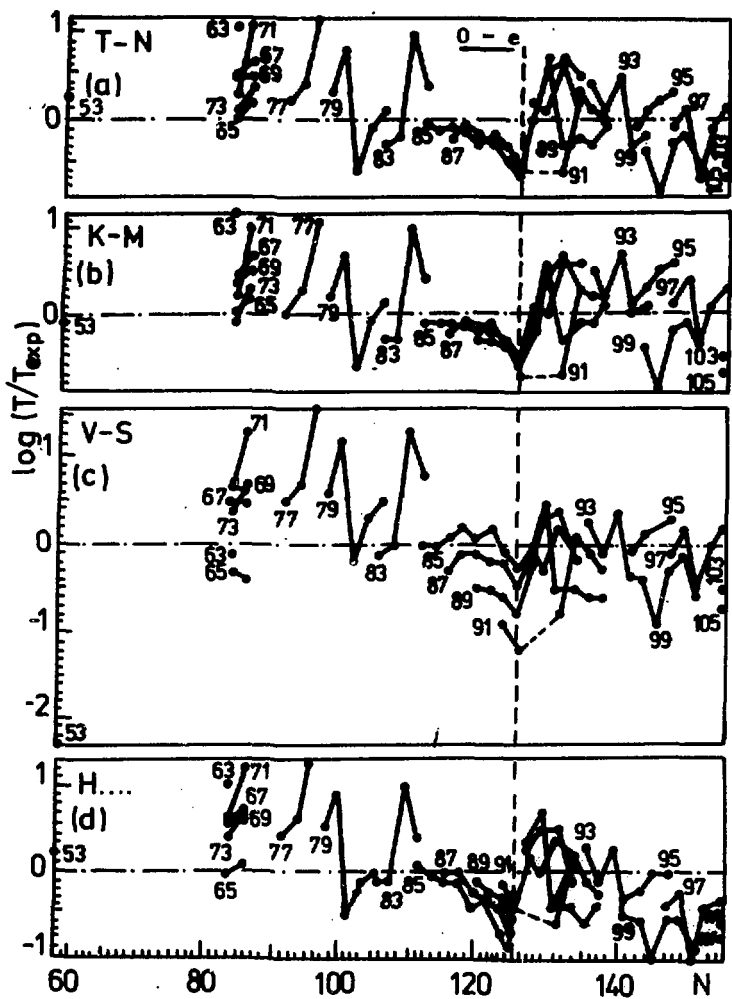
Fig.3. The same as Fig. 2 for odd-even nuclei.
