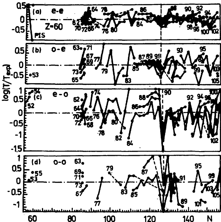
Fig.5. The errors of life-time prediction with our formula when X is approximated with a second order polynomial of two variables for even-even (a), odd-even (b), even-odd (c), and odd-odd nuclei (d).
