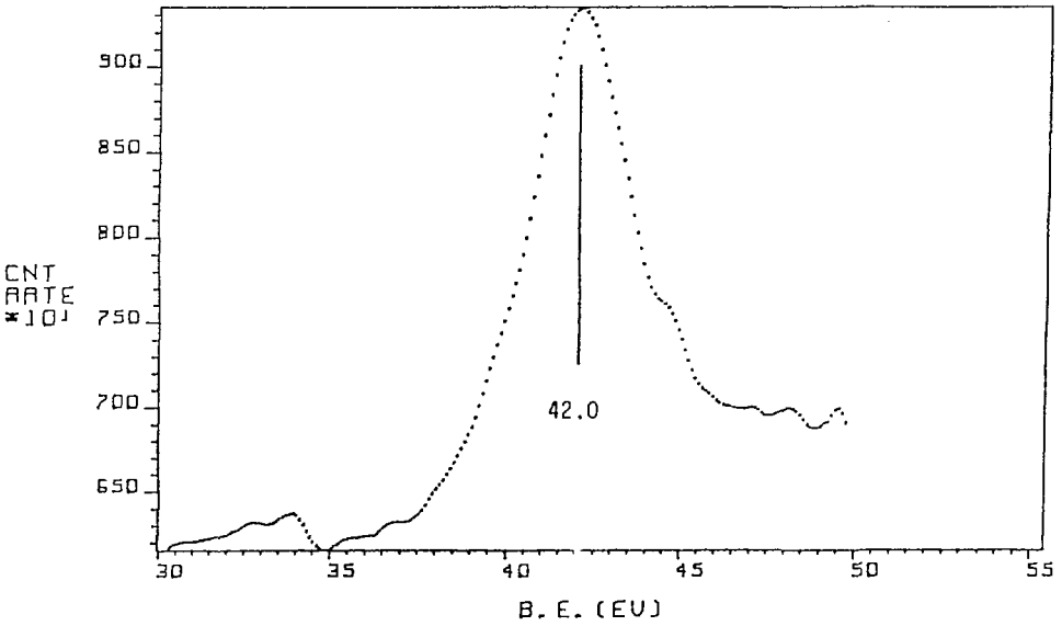
Fig. 46 V3p XPS spectrum of V 2 O 5 .
