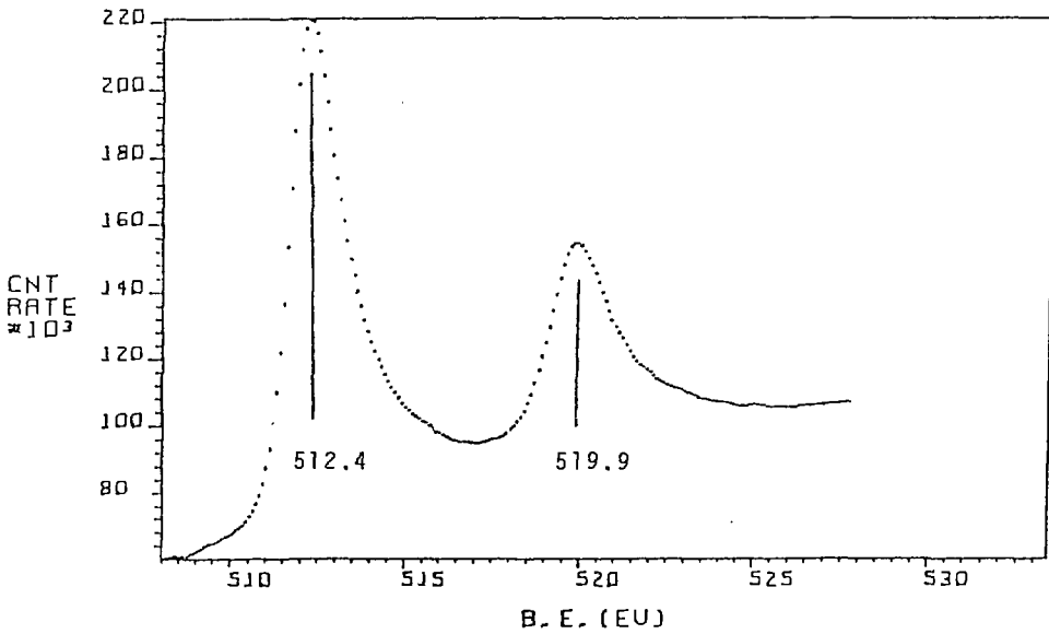
Fig. 40 V_{2p} XPS spectrum of V_{et} .
