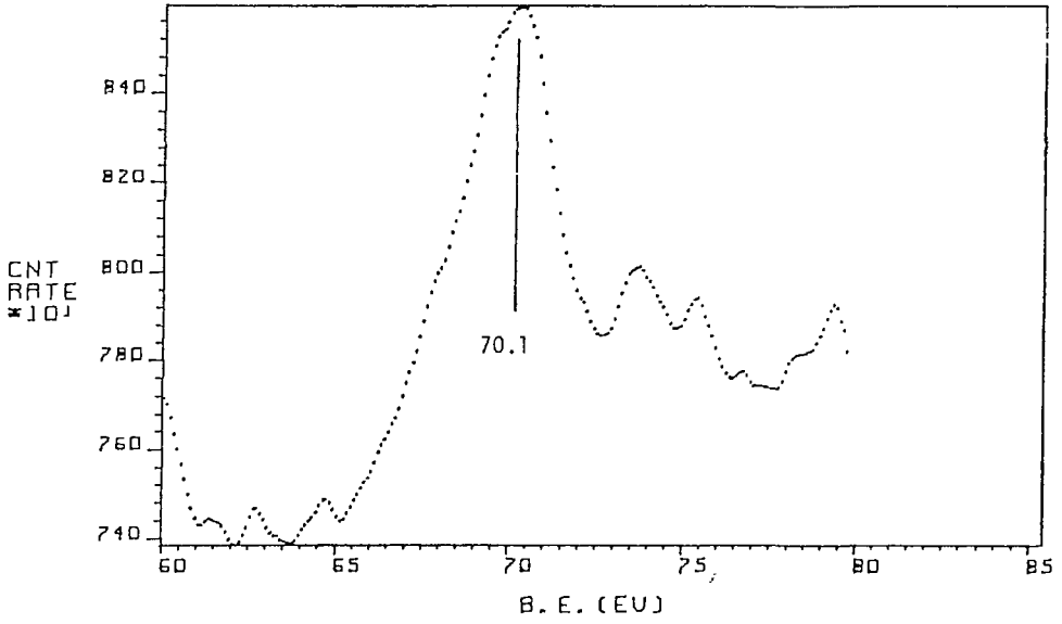
Fig. 45 V3s XPS spectrum of V 2 O 5 .
