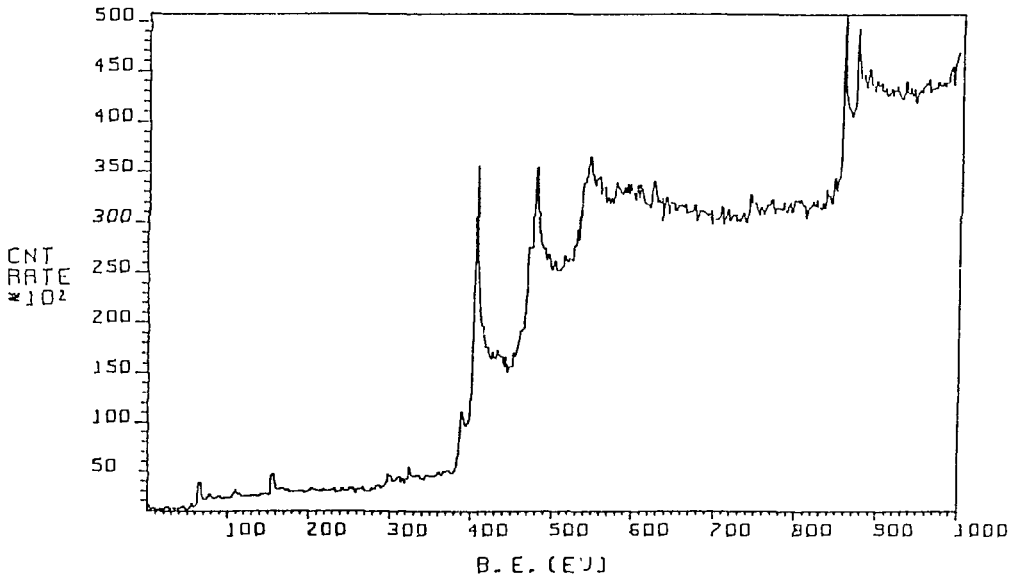
Fig. 50 XPS wide scan of Ni_{fz} .
