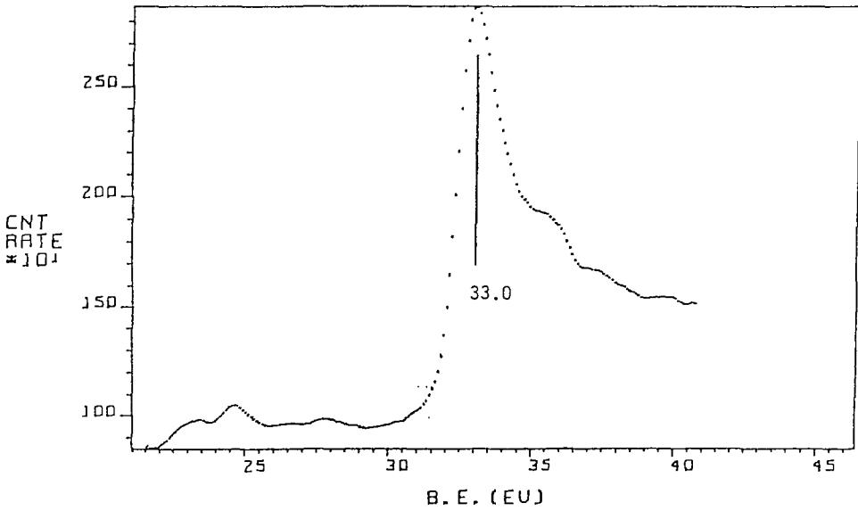
Fig. 22 Ti3p XPS spectrum of Ti fl .
