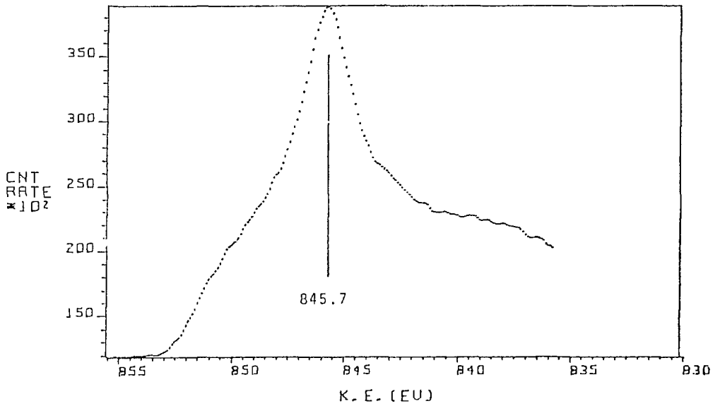
Fig. 53 L_3M_{2,3}M_{2,3} XAES spectrum of Ni_{f2} .
