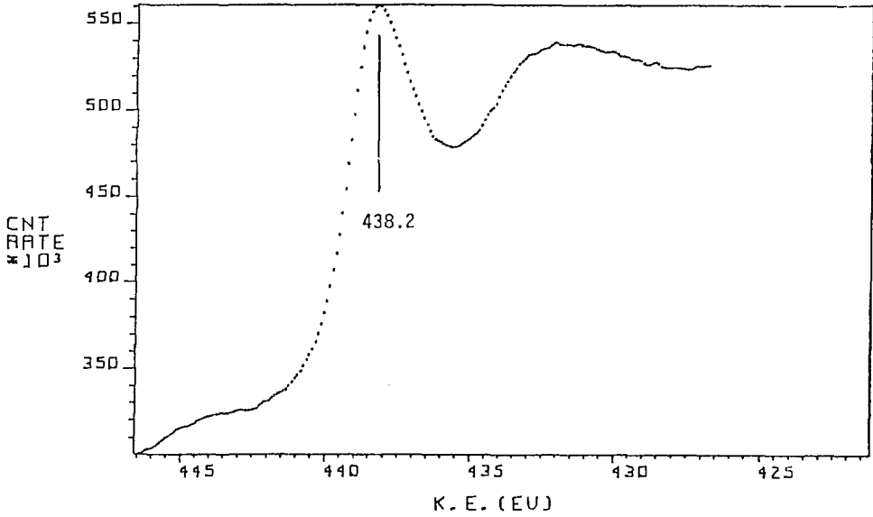
Fig. 39 L_{3}M_{2,3}V XAES spectrum of V_{fz} .
