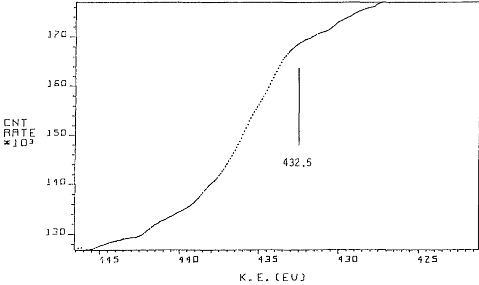
Fig. 49 L_{3M_{2,3}V} XAES spectrum of V_2O_5 .
