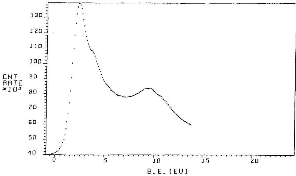
Fig. 59 Valence-band spectrum of NiO.
