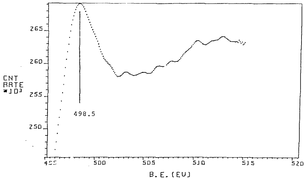
Fig. 2 Sc 2s XPS spectrum of Sc fl .
