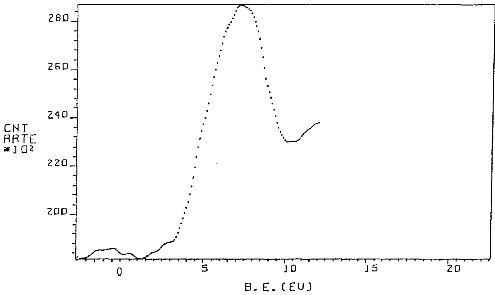
Fig. 16 Valence-band spectrum of Sc 2 O 3 .
