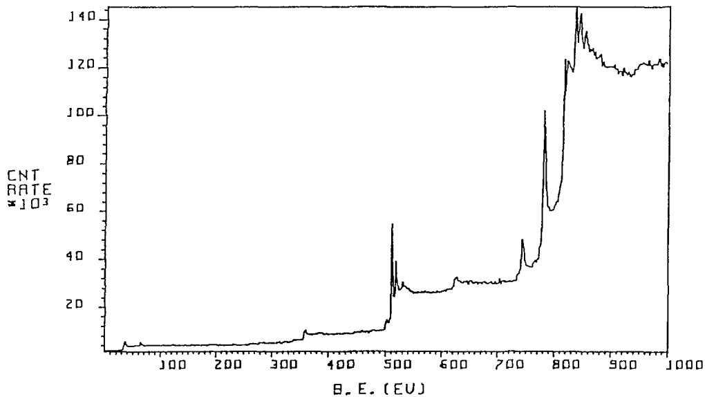
Fig. 33 XPS wide scan of V_{fl} .
