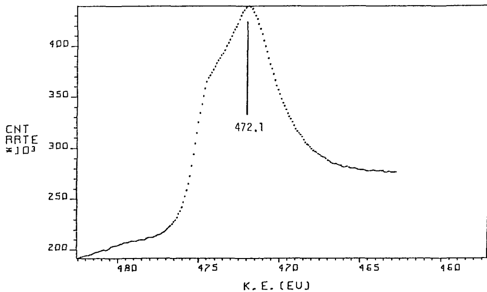
Fig. 38 L_{3}M_{2,3}M_{2,3} XAES spectrum of V_{fi} .
