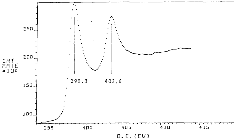
Fig. 3 Sc2p XPS spectrum of Sc fl.
