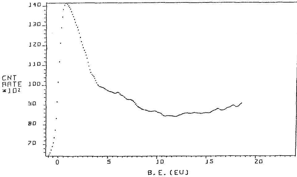
Fig. 52 Valence-band spectrum of Ni fz .
