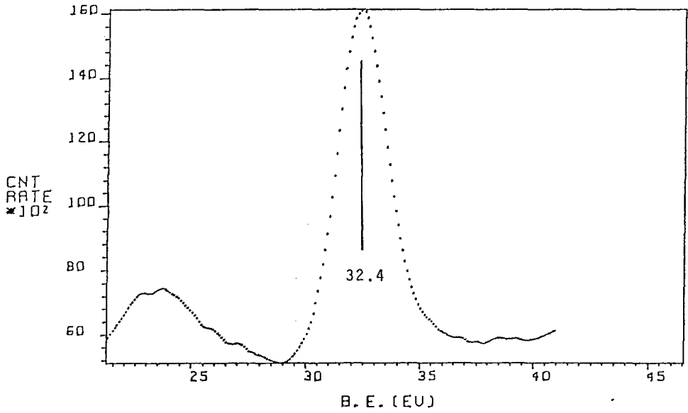
Fig. 15 Sc 3p XPS spectrum of Sc 2 O 3 .
