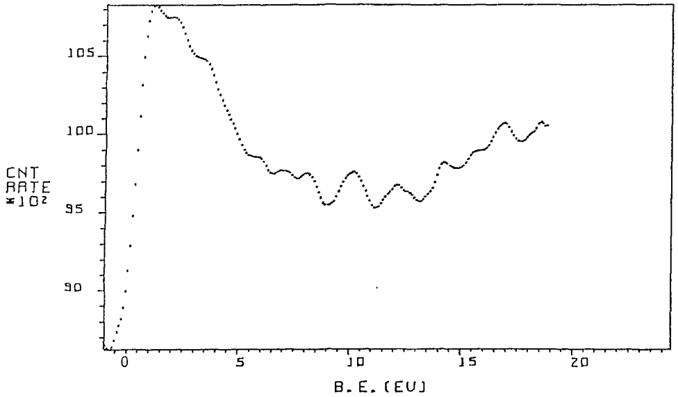
Fig. 23 Valence-band spectrum of Ti fl .
