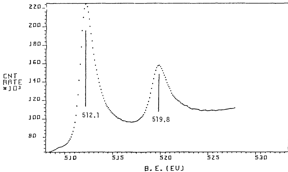
Fig. 34 V2p XPS spectrum of V_{fl} .
