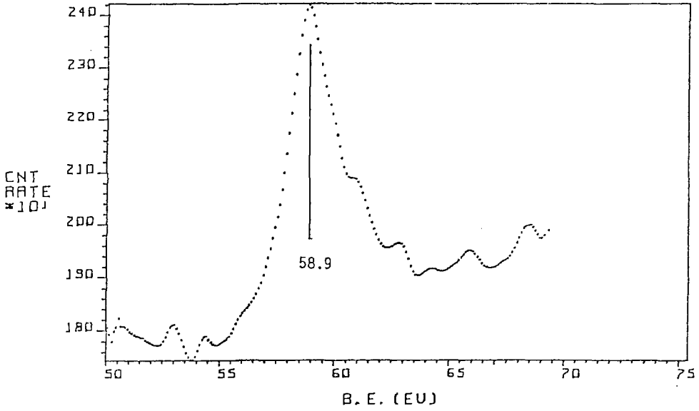
Fig. 21 Ti3s XPS spectrum of Ti fl .
