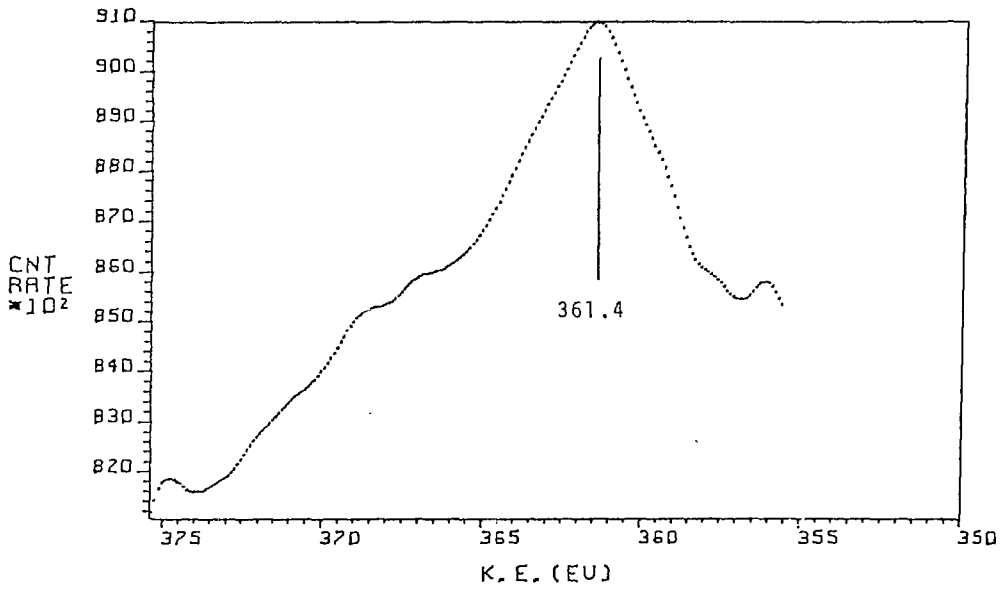
Fig. 18 L_{2,3}M_{2,3}V XAES spectrum of Sc_2O_3 .
