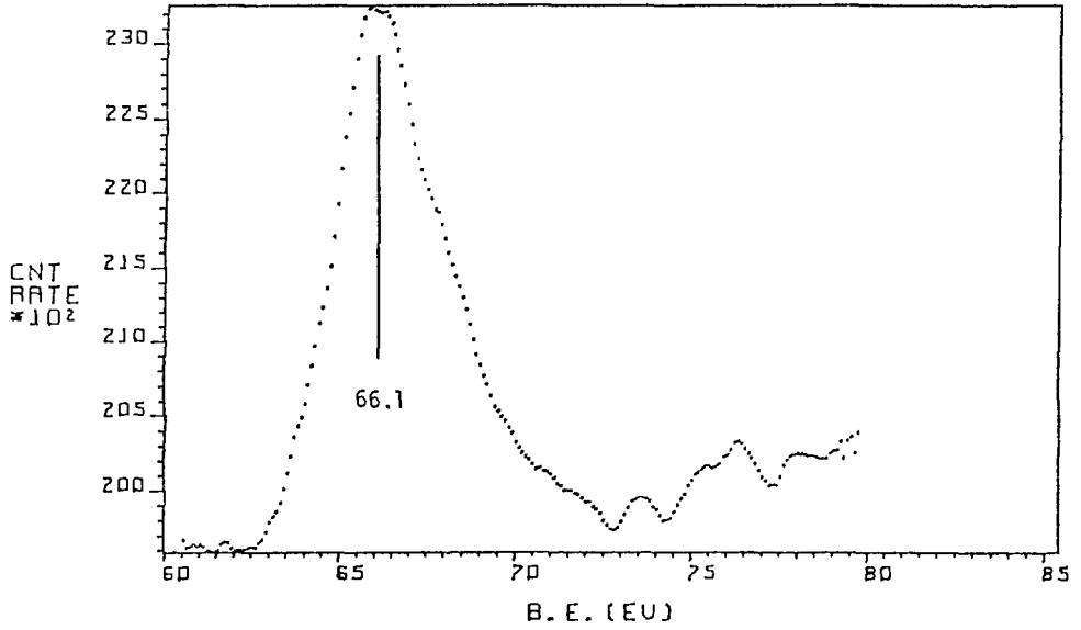
Fig. 35 V3s XPS spectrum of V_{fz} .
