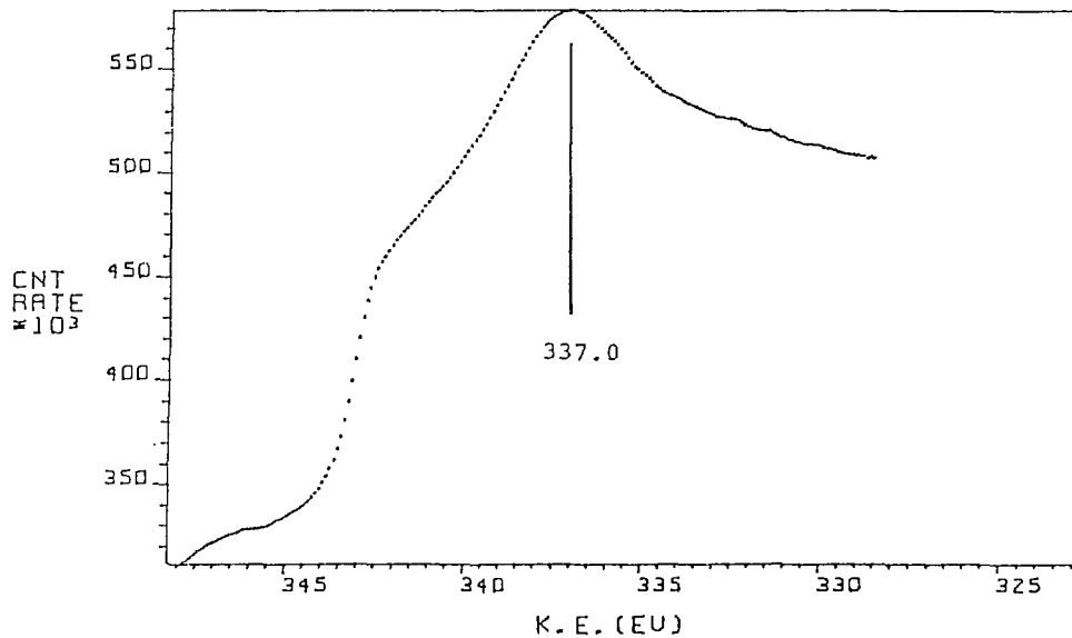
Fig. 7 L_{2,3}M_{2,3}M_{2,3} XAES spectrum of Sc fl .
