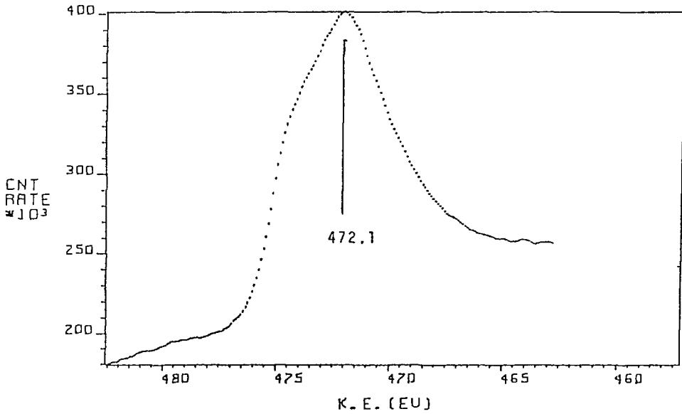
Fig. 42 L_{3}M_{2,3}M_{2,3} XAES spectrum of V_{et} .
