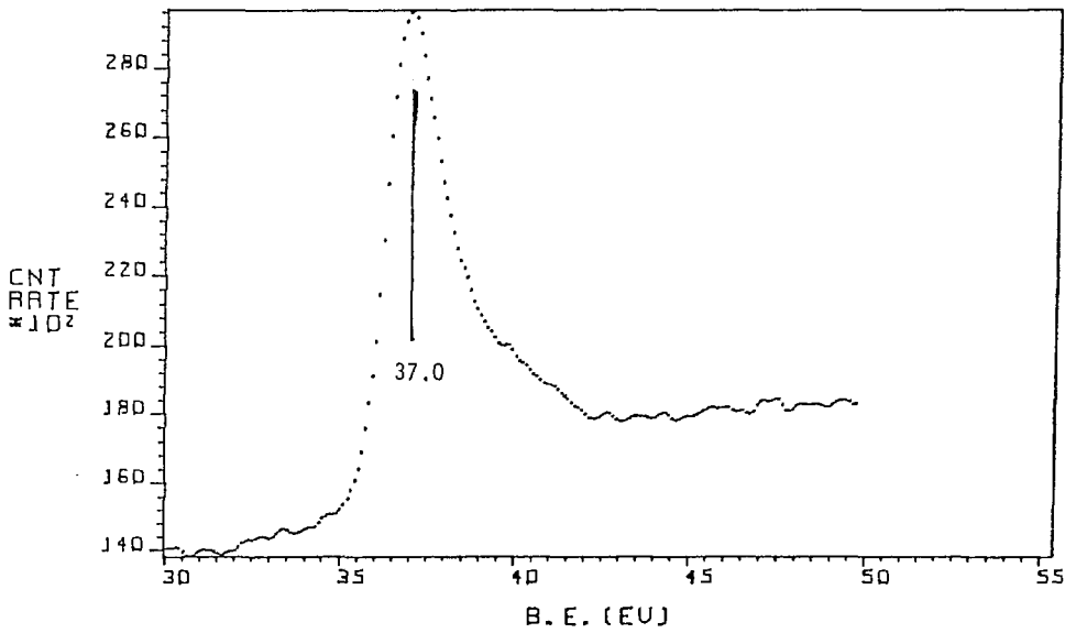
Fig. 36 V3p XPS spectrum of V_{fz} .
