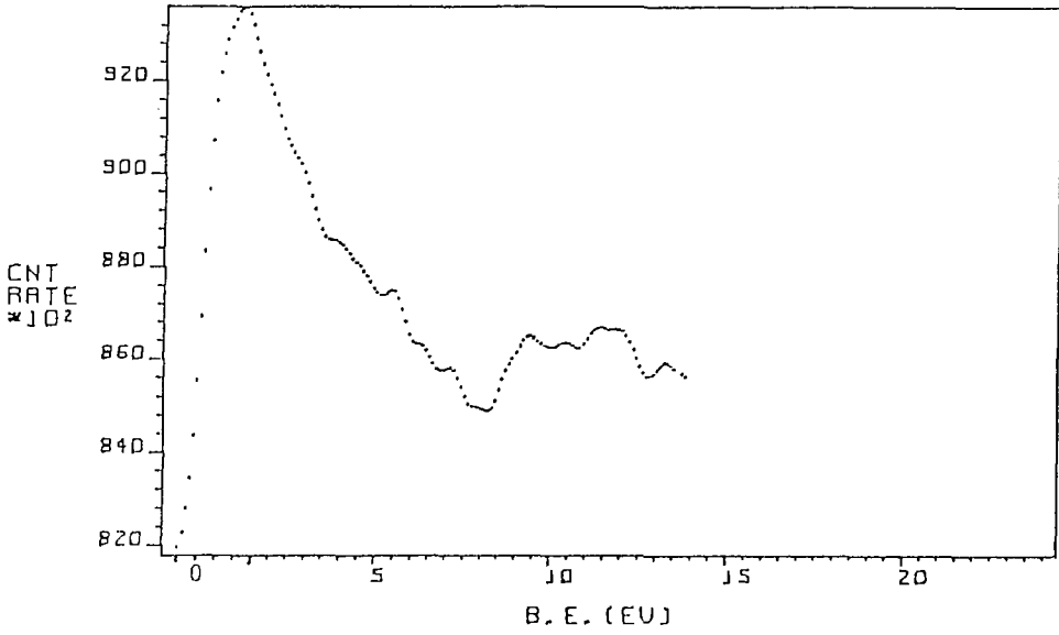
Fig. 41 Valence-band spectrum of V_{et} .
