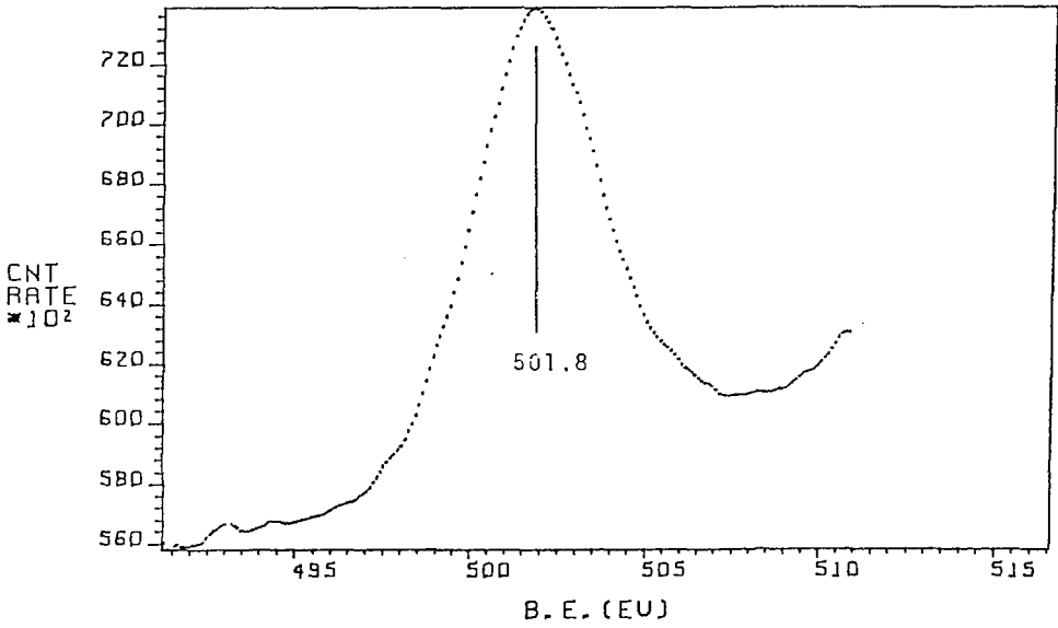
Fig. 12 Sc 2 s XPS spectrum of Sc 2 O 3 .
