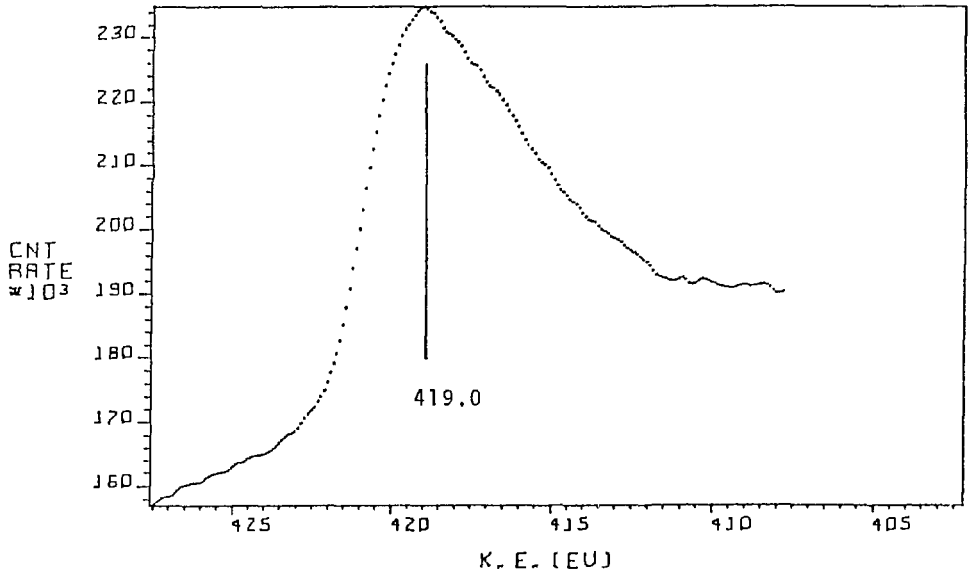
Fig. 27 L_{2,3}M_{2,3}V XAES spectrum of Ti_{et} .
