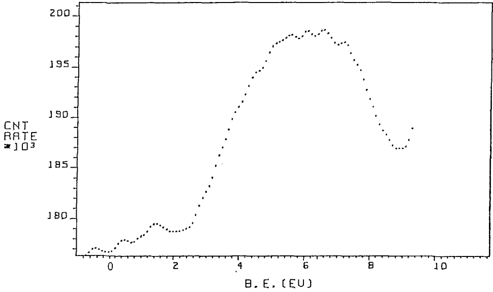
Fig. 47 Valence-band spectrum of V 2 O 5 .
