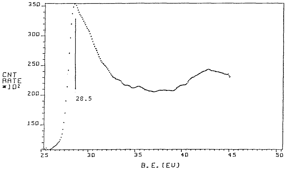
Fig. 5 Sc 3p XPS spectrum of Sc fl.
