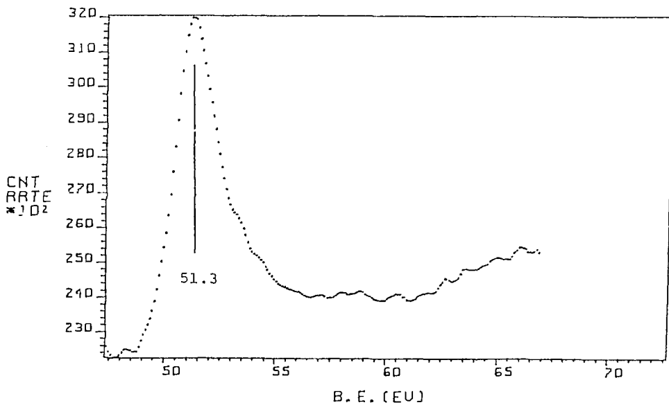
Fig. 4 Sc3s XPS spectrum of Sc fl.
