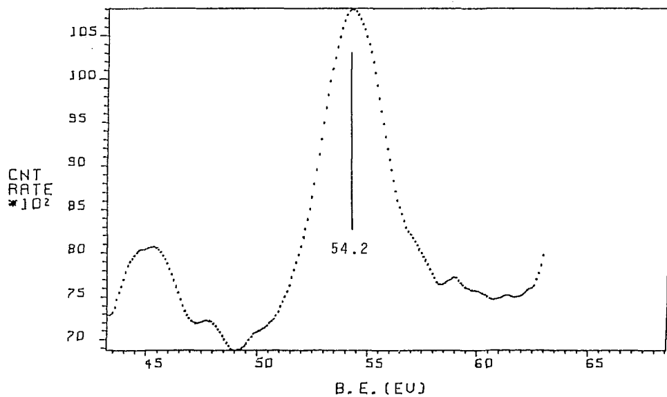
Fig. 14 Sc 3 s XPS spectrum of Sc 2 O 3 .
