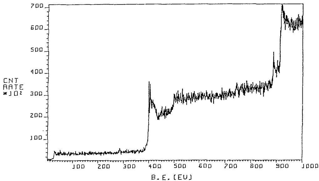
Fig. 1 XPS wide scan of Sc fl .
