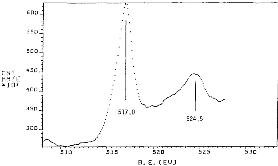
Fig. 44 V_{2p} XPS spectrum of V_2O_5 .
