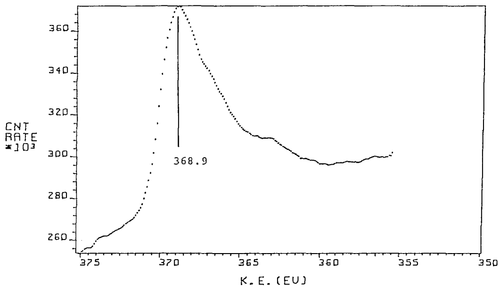
Fig. 8 L_{2,3}M_{2,3}V XAES spectrum of Sc fl .
