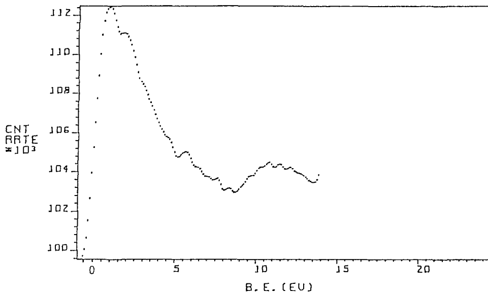
Fig. 37 Valence-band spectrum of V_{fi} .
