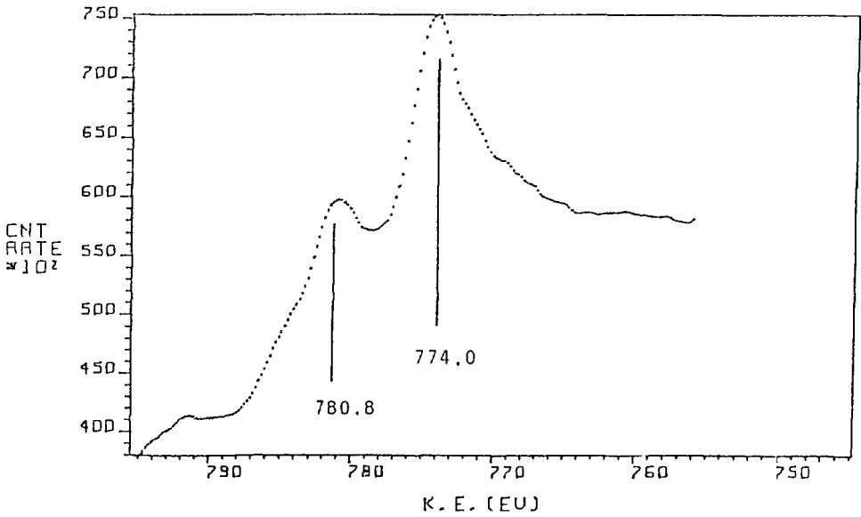
Fig. 54 L_3M_{2,3}V XAES spectrum of Ni_{f2} .
