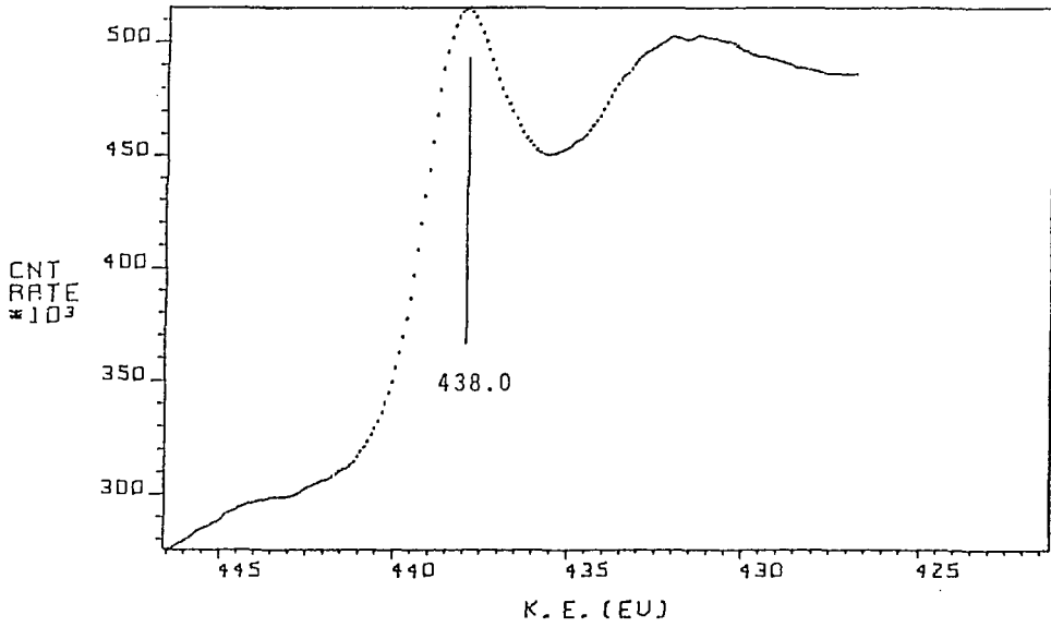
Fig. 43 L_{3}M_{2,3}V XAES spectrum of V_{et} .
