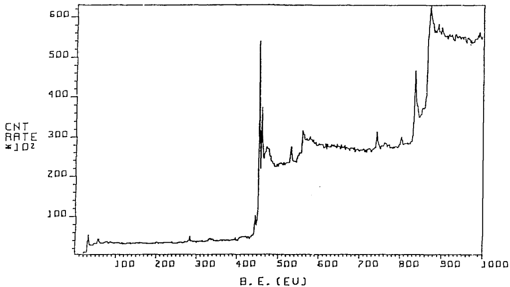
Fig. 19 XPS wide scan of Ti fl .
