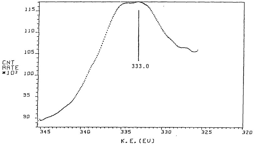
Fig. 17 L_{2,3}M_{2,3}M_{2,3} XAES spectrum of Sc_2O_3 .
