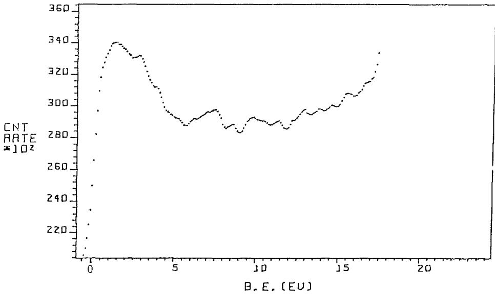
Fig. 6 Valence-band spectrum of Sc fl.
