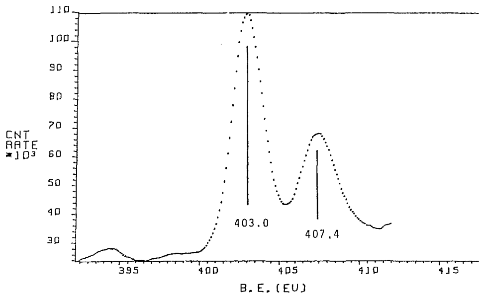
Fig. 13 Sc 2 p XPS spectrum of Sc 2 O 3 .
