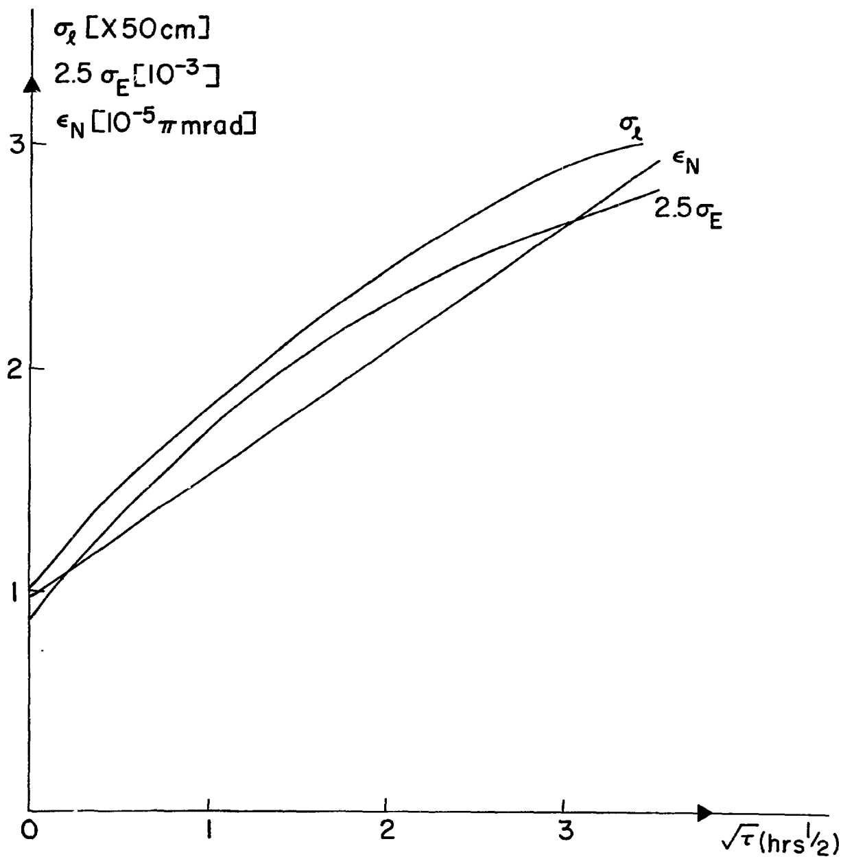
Fig. 1 Bunch length, energy spread and the normalized emittance of the beam par-
