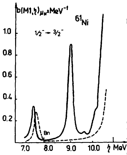
Fig.2. Strength functions of the M1 transitions in ^{61}\text{Ni} from p-wave resonances with J^\pi = 1/2^- to the ground state with J^\pi = 3/2^- . Notation: solid line is the calculations allowing for the function U_{\lambda_2^{i_1}}^{\lambda_1^{i_1}}(J_1) (formula (5)), dashed line is the calculations disregarding U_{\lambda_2^{i_1}}^{\lambda_1^{i_1}}(J_1) .
