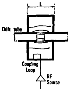
Fig. 3 - single gap accelerating structure
