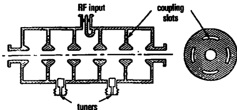
Fig. 8 - Nose cone structure
