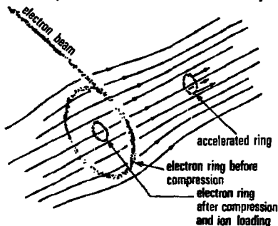
Fig. 12 - Principle of the Electron Ring Accelerator (ERA)
