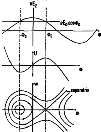
Fig. 21 - Phase stability graphs
