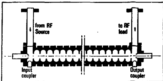
Fig. 7 - Travelling wave accelerating structure
