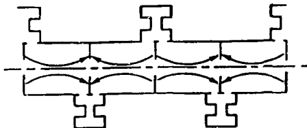
Fig. 9 - Side coupled structure
