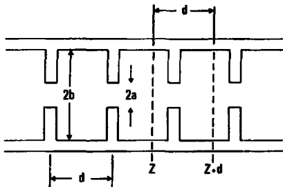
Fig. 17 - Periodic loaded structure
