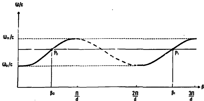
Fig. 18 - Brillouin diagram for a slow wave structure
