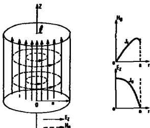
Fig. 15 - TM_{010} mode in a pill-box cavity
