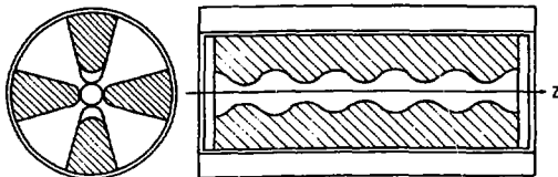
Fig. 11 - Schematic drawing of an RFQ resonator
