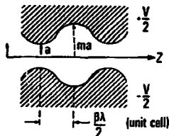
Fig. 23 - Modulated pole shapes in an RFQ
