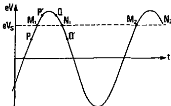
Fig. 20 - Particle phases relative to the RF field
