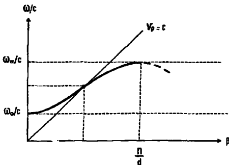
Fig. 19 - Operating point for v_p = c
