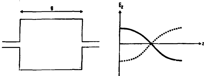
Fig. 14 - TM_{011} mode in a pill-box cavity
