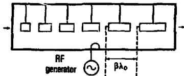
Fig. 5 - ALVAREZ type structure
