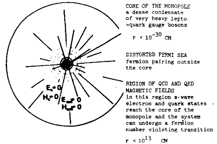
Fig.3 depicts a monopole.
