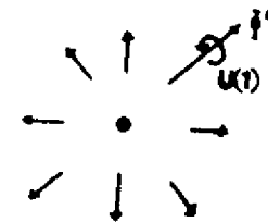
Fig.2 - Hedgehog configuration of Higgs field around a monopole
