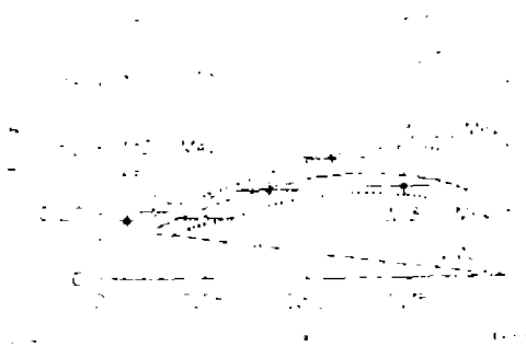
Fig. 6. Analysis of the photon structure function in the Antoniadis-Grunberg scheme. 37) See the reviews of A. Deuter and W. Wagner, these proceedings.
