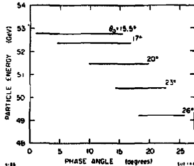
Fig. 4. Particle energy along bunches of Fig. 3 as a function of phase angle.
