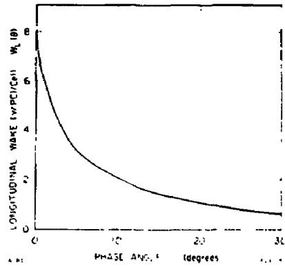
Fig. 1. Longitudinal wake function w_L(\theta) for single average cavity of SLAC constant-gradient structure.
