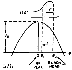
Fig. 2. Definitions of phase angles showing position of bunch with respect to accelerating wave. The charge distribution is f(\theta') and the maximum energy gain is V_0 .
