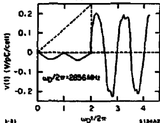
Fig. 2. A triangular bunch in the SLAC structure.
