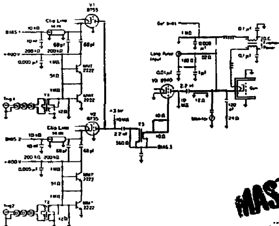
Fig. 1. Schematic diagram of the fast double pulser.
