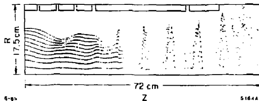
Figure 3. Electron density plot for the 50 MW klystron.
