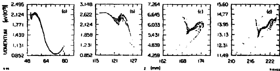
Figure 2. Longitudinal phase space as a function of Z for the bunch shown in Figure 1.
