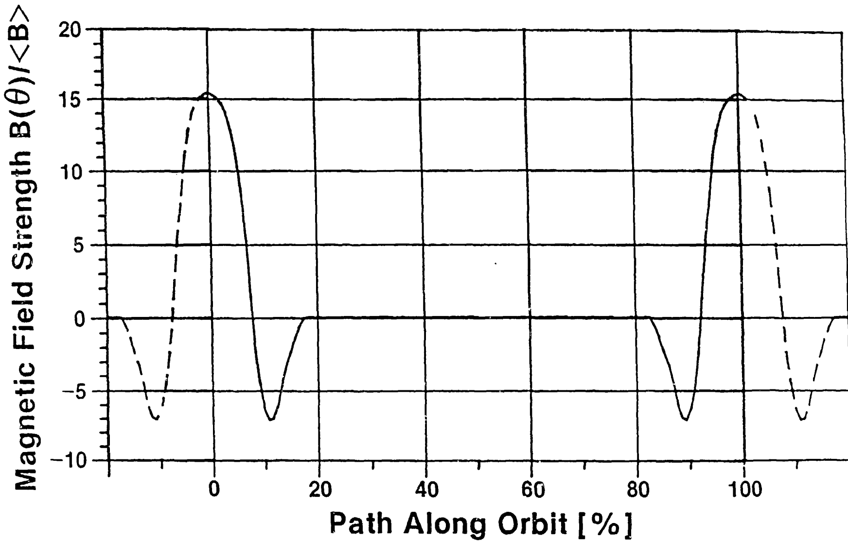
Fig. 3. The azimuthal profile of the magnetic field along one lattice cell.
