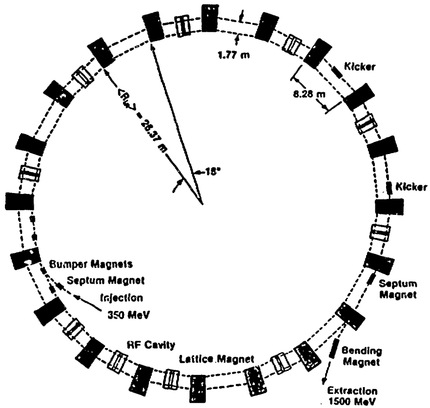
Fig. 2. Schematic view of the 1500-MeV FFAG, radial type.
