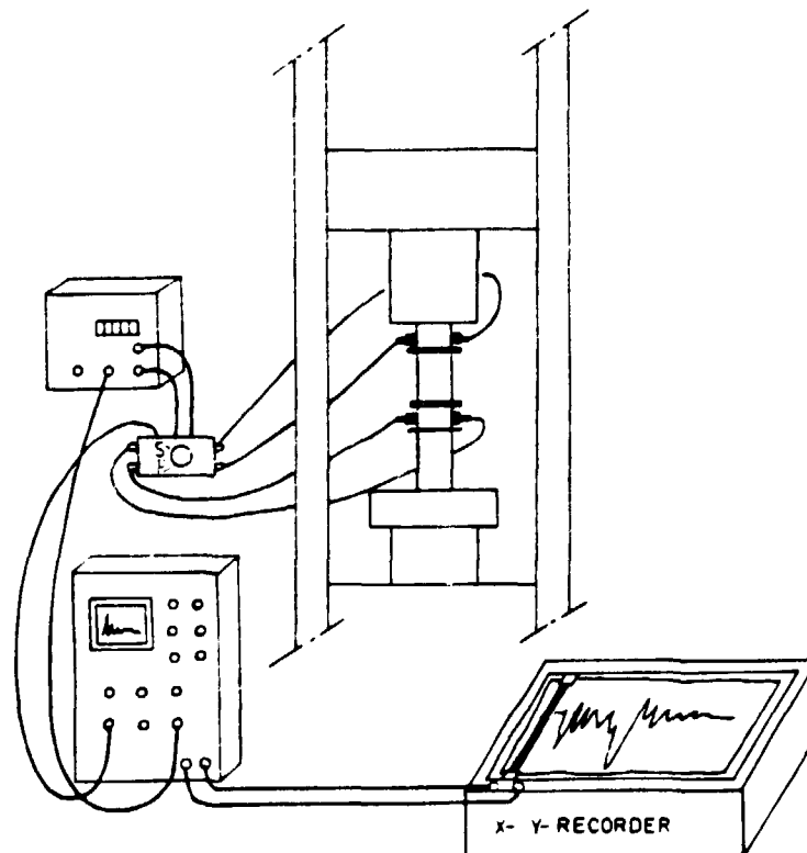
Fig. 1 The layout of components for measuring sound velocity in rock specimens.
