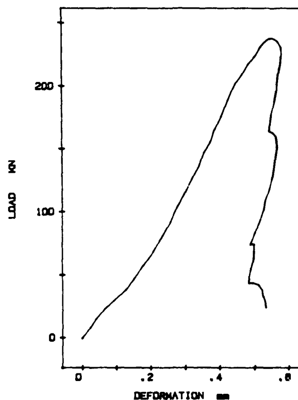
Figure 3-5 A typical load-deformation curve at a confining pressure of 10 MPa. Sample Gid 3(10).
