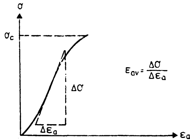
Fig. 4 Calculation of the average modulus of elasticity.
