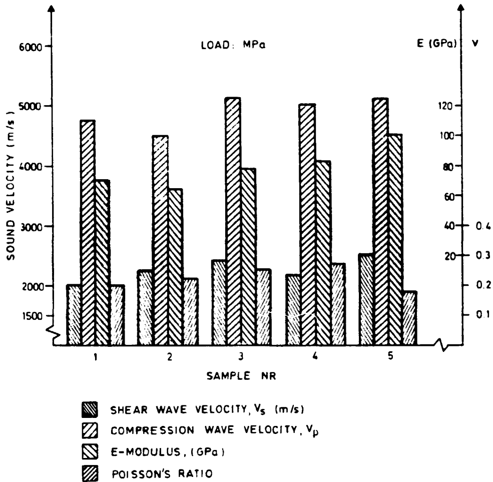
Fig. 4 Sample comparison diagram for each specimen showing: V_s (m/s), V_p (m/s), Young's modulus (GPa) and Poisson's ratio.
