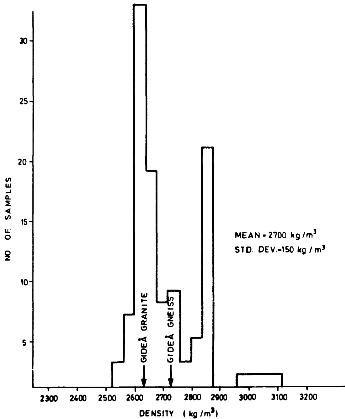
Figure 4-1 Frequency histogram of density of crystalline rocks. 104 samples. Gideå results are indicated by the arrows. (After Tammemagi and Chieslar, 1985).
