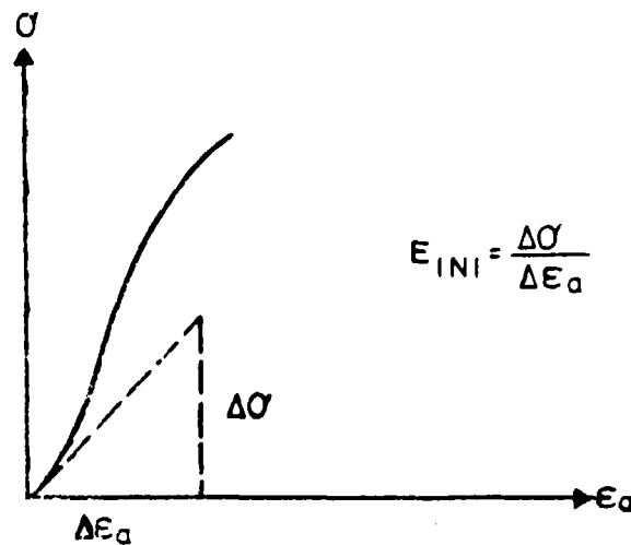
Fig. 6 Calculation of the initial modulus of elasticity.
