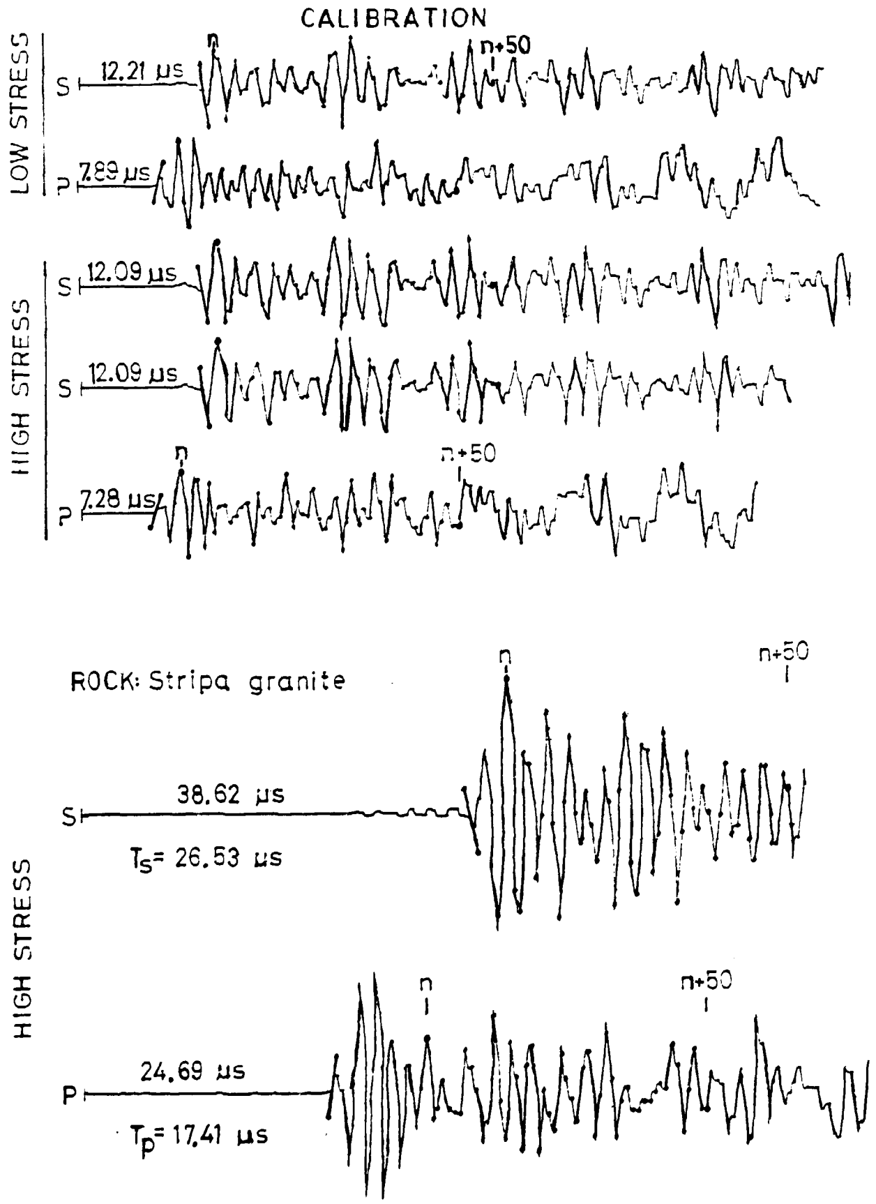
Fig. 3 Typical plots from P- and S-waves in Stripa Granite.
