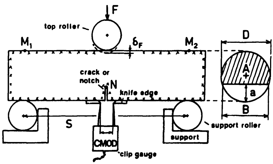
Fig 1 Experimental set-up for three point bending test.
