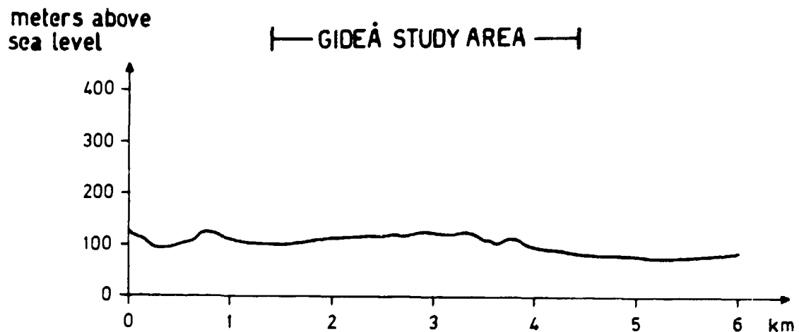
Figure 2-2 Topographic profile through the Gideå study area. Profile is east - west striking.
