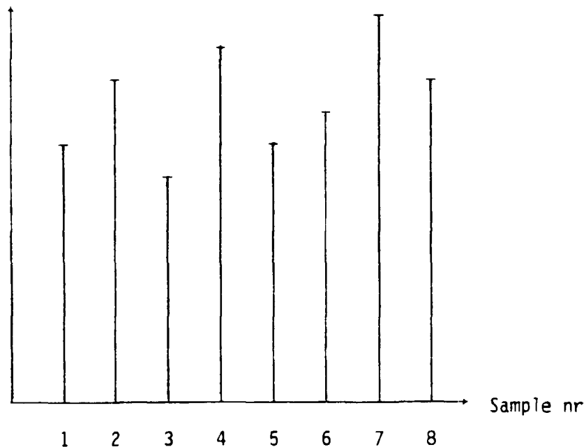
Fig. 8 Example of a sample-comparison diagram showing the variation of compressive strength between specimens in the same series.
