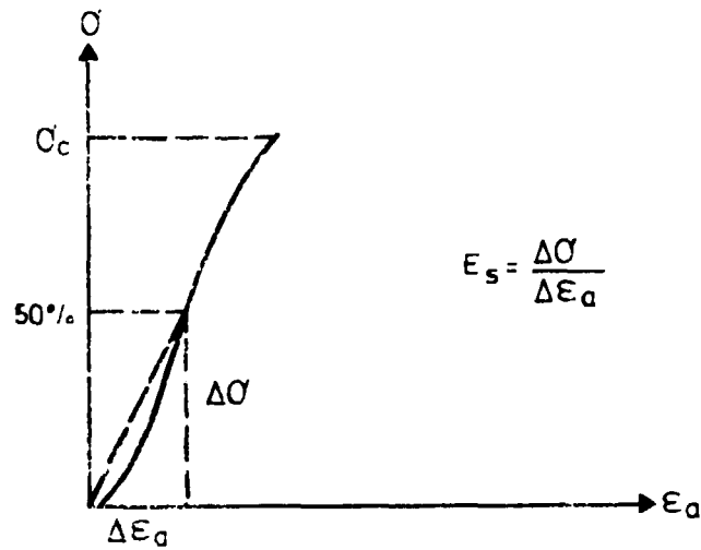
Fig. 5 Calculation of the secant modulus of elasticity.
