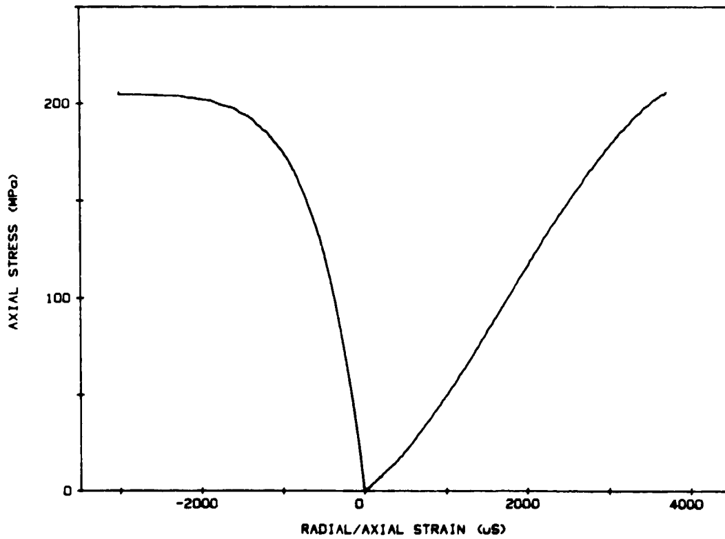
Figure 3-2 Stress versus radial/axial deformation A) migmatitic gneiss, B) migmatitic granite
