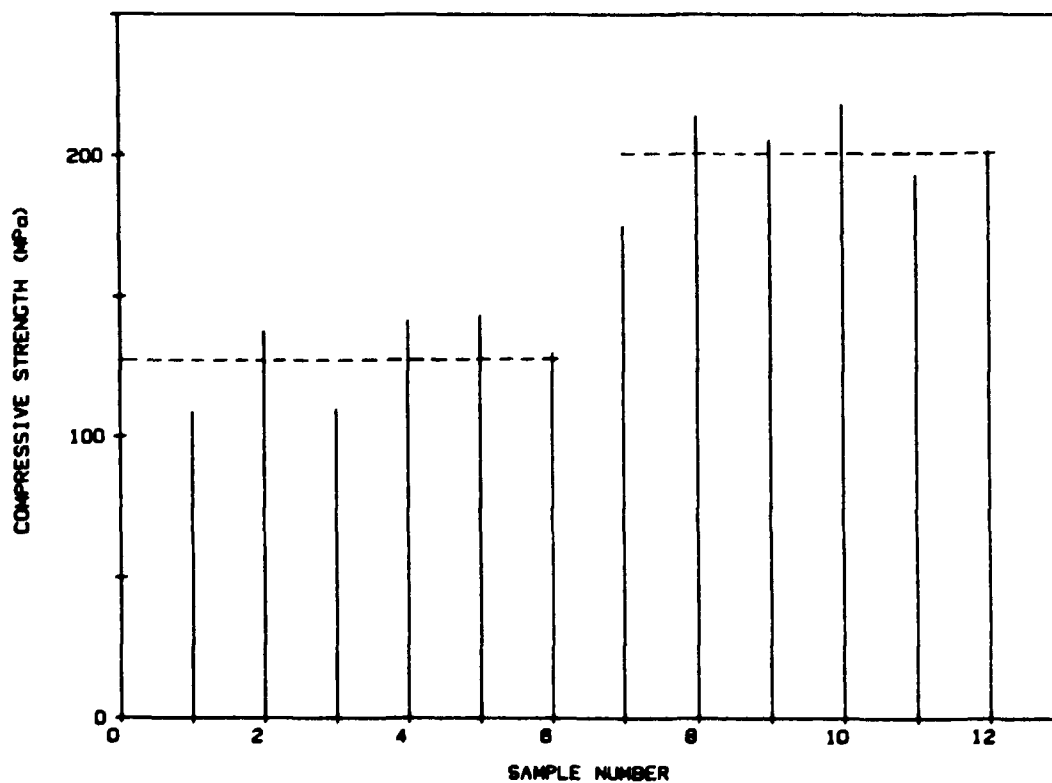
Figure 3-1 Results from uniaxial compression tests. Sample number 1-6: migmatitic gneiss, sample number 7-12: migmatitic granite. The dotted line indicates the average value for each rock type.
