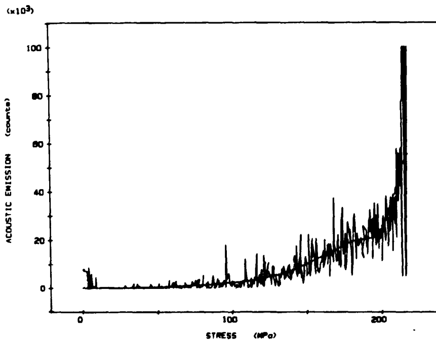
Figure 3-3 Acoustic emission versus axial stress for uniaxial compression test. A: migmatitic gneiss, B: migmatitic granite
