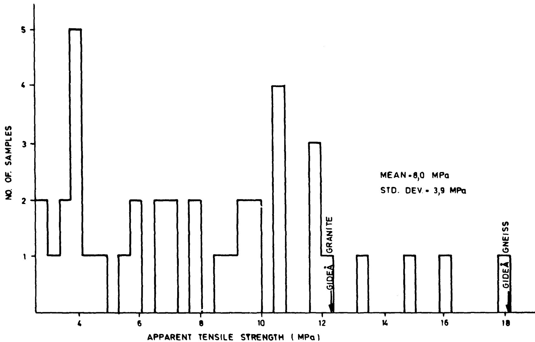
Figure 4-5 Frequency histogram of apparent tensile strength for crystalline rocks. 39 samples. Gideå results are indicated by the arrows. (After Tammemagi and Chieslar, 1985).
