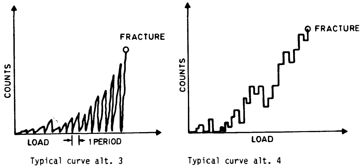
Fig 2 Typical curves for the different registering alternatives.
