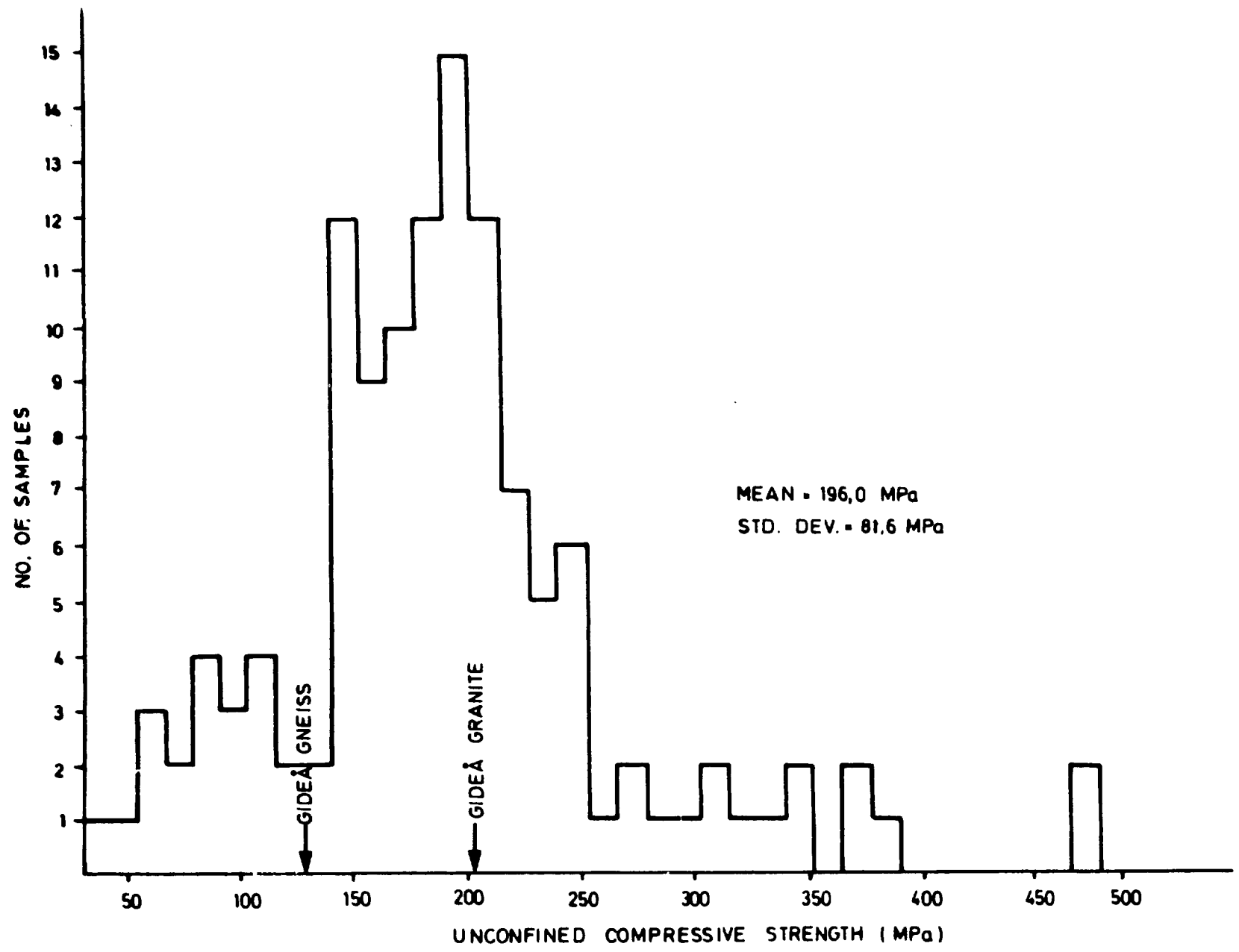
Figure 4-4 Frequency histogram of unconfined compressive strength for crystalline rocks. 127 samples. Gideå results are indicated by the arrows. (After Tammemagi and Chieslar, 1985).
