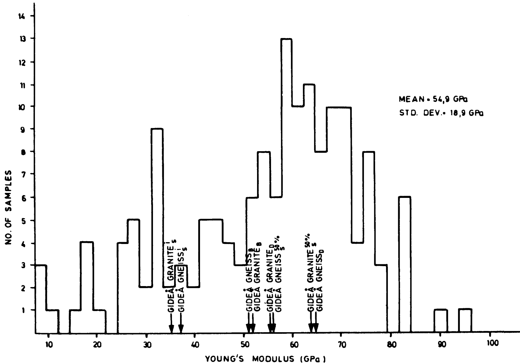
Figure 4-2 Frequency histogram of Young's modulus for crystalline rocks. 160 samples. Results from Gideå are indicated by the arrows. (After Tammemagi and Chieslar, 1985).
