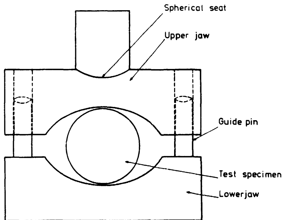
Fig 1 Loading equipment for Brazilian test.
