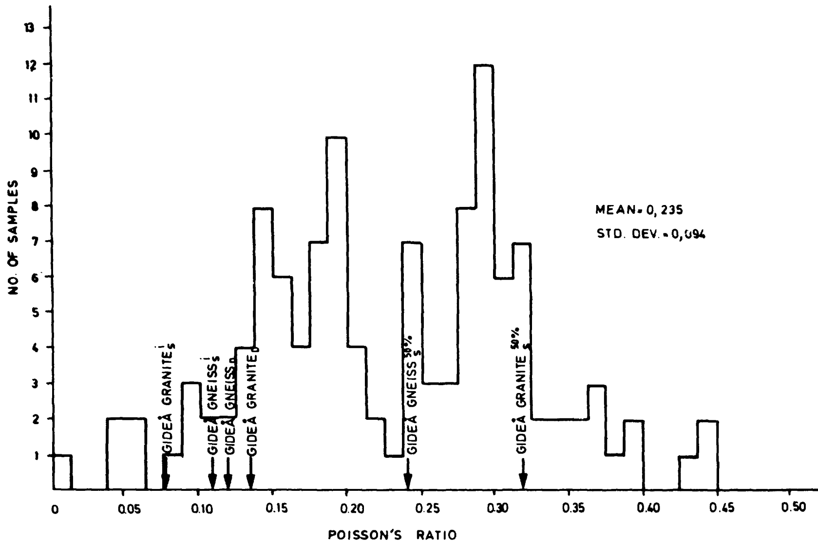
Figure 4-3 Frequency histogram of Poisson's ratio for crystalline rocks. 121 samples. Results from Gideå are indicated by the arrows. (After Tammemagi and Chieslar, 1985).
