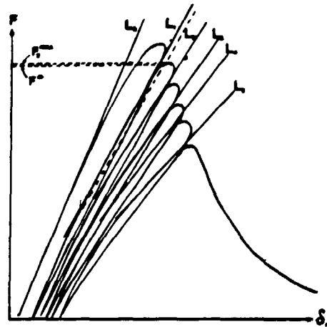
Fig 3 Diagram of load, F , as function of load point deformation, \delta_F , for a cyclic test.
