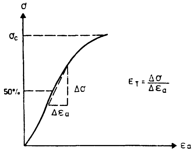
Fig. 3 Calculation of the tangent modulus of elasticity.
