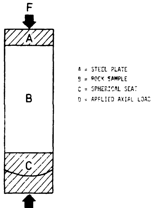
Fig. 1 Example of an experimental set-up.
