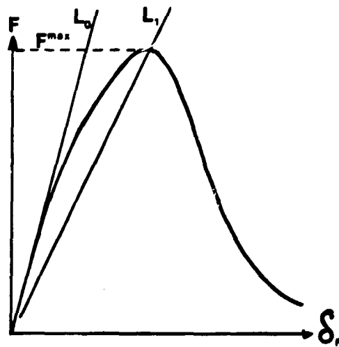
Fig 2 Diagram of load, F, as function of load point deformation, \delta_F , for a test with one cycle.
