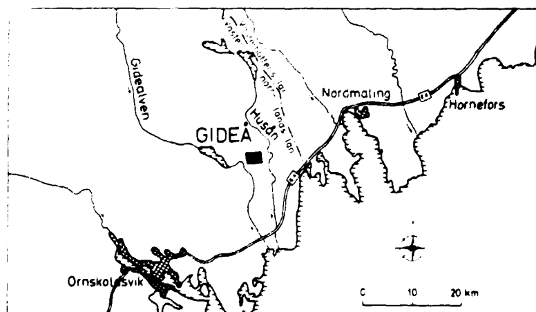
Figure 2-1, Overview map of the Gideå study area
