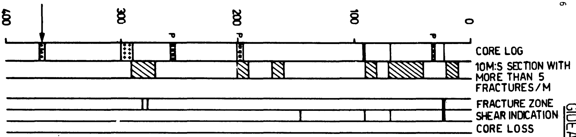
Figure 2-3 Summary of core mapping for drillhole Gt 1. Arrows indicate from which depths the test samples were taken. After Albino, et. al., 1982
