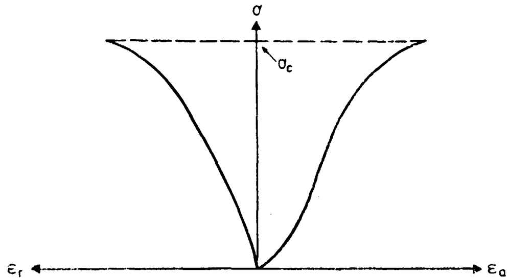
Fig. 2 Example of a graphical presentation of axial and radial stress-strain curves.
