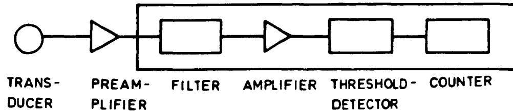
Fig 1 Block diagram for AE equipment.
