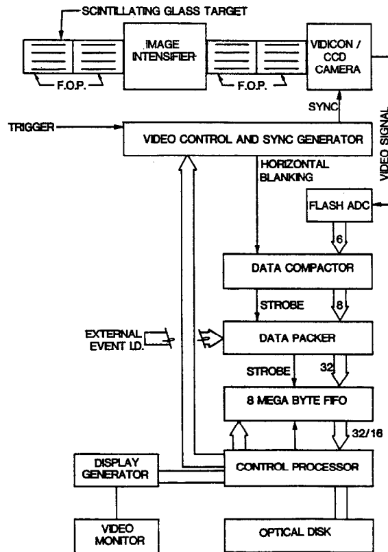
Fig.1 Overview of Video-Data-Aquisition system to be used in Fermilab Experiment E-687.
