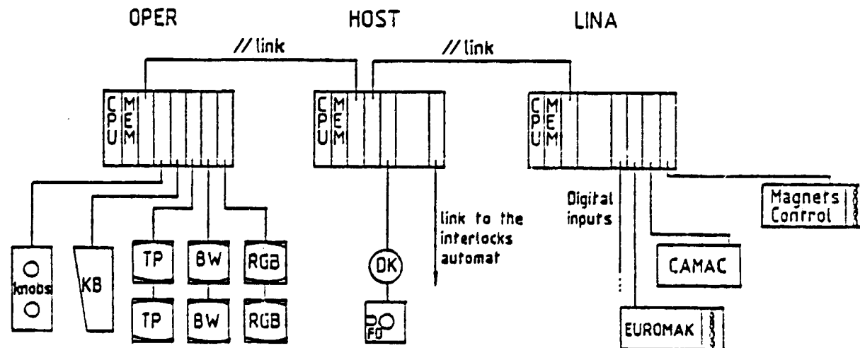
Hardware Configuration
