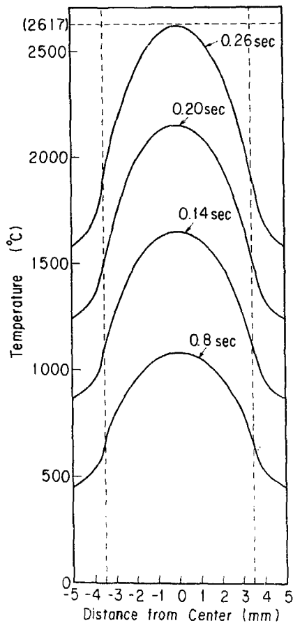
Fig. 9 Temperature gradient of the sample during the hydrogen beam irradiation
