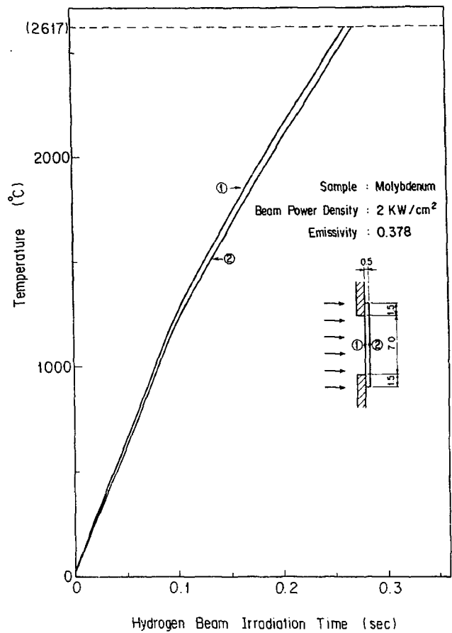
Fig. 10 Temperature of the sample during the hydrogen beam irradiation
