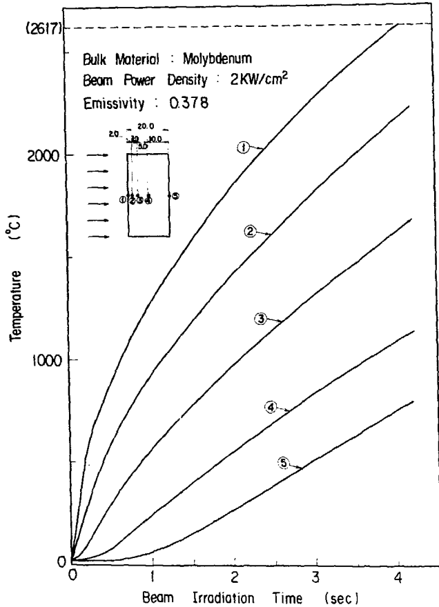
Fig. 11 Temperature distribution of the molybdenum plate (20 mm) during the beam irradiation
