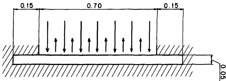
Fig. 8 Calculation model for the thermal analysis
