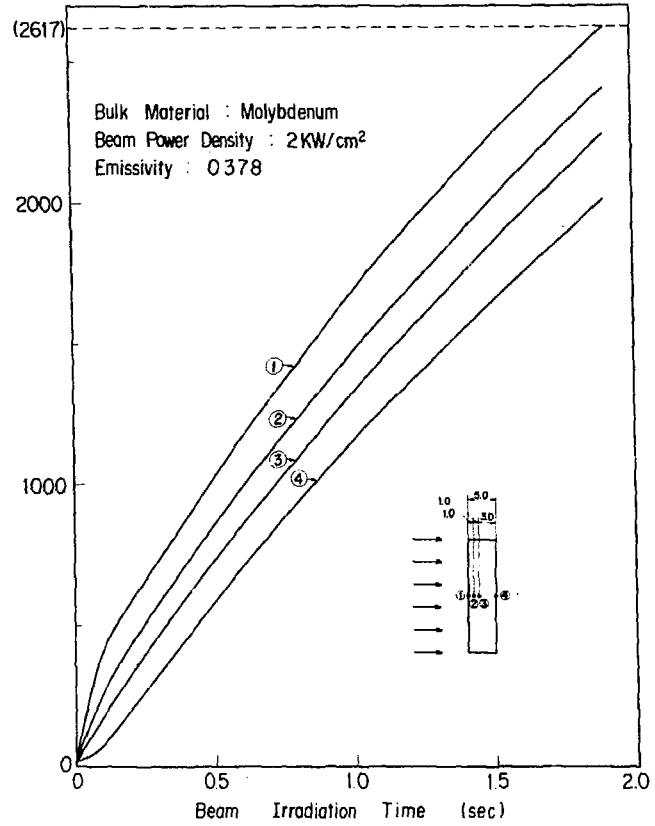
Fig. 12 Temperature distribution of the molybdenum plate (5 mm) during the beam irradiation
