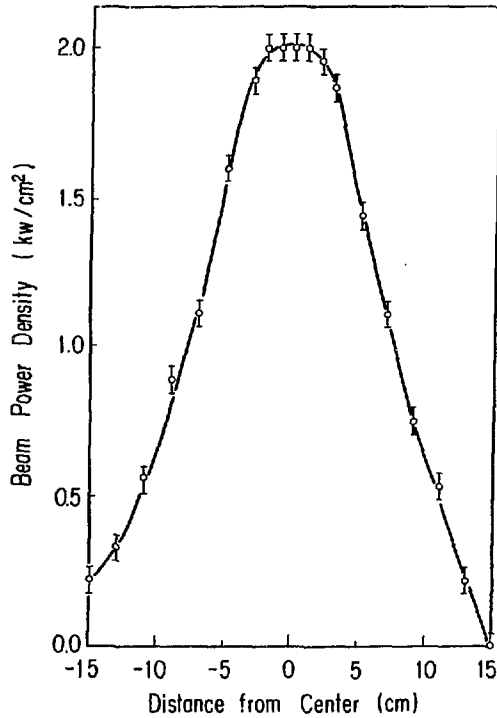
Fig. 2 Power density distribution of the hydrogen beam
