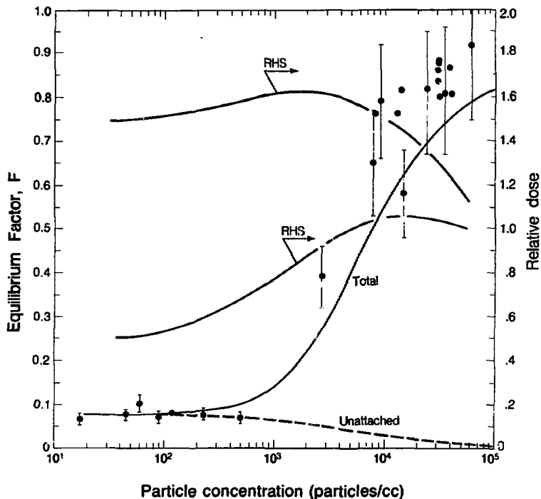
Figure 7. Equilibrium factor, F , versus particle concentration. Measured data and representative uncertainties are indicated by the solid circles and error bars. The solid line labelled Total represents calculated values of F for total airborne radon progeny concentrations while the dashed line indicates calculated F values for unattached radon progeny only (see text). The relative dose curves, which refer to the right axis (RHS), are for children undergoing light activity (upper curve) and adults at rest (lower curve). These relative dose curves should be regarded as illustrative, rather than accurate dosimetric predictions.
