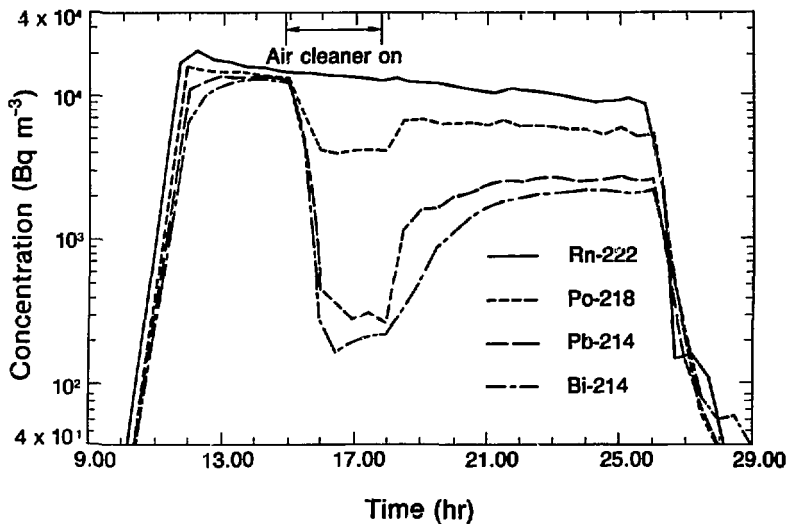
Figure 3. Radon and radon progeny concentration as a function of time. The effect of operation of the HEPA-type filter is indicated. The sharp decrease in radon and radon progeny concentrations shown in the figure is due to ventilation of the test space at the end of the experiment.
