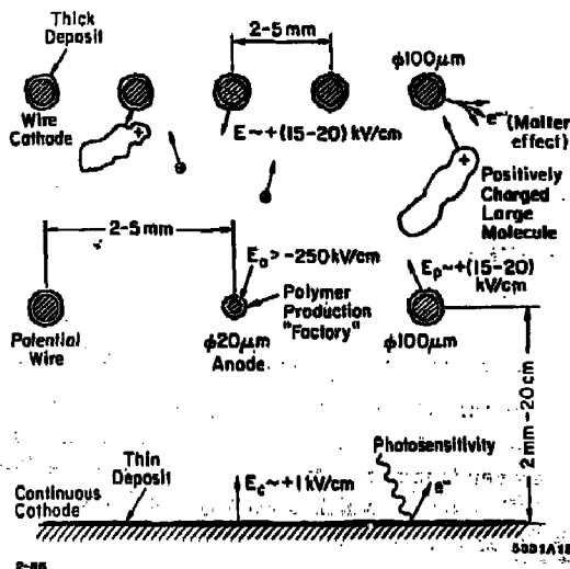
Fig. 16. Typical wire chamber structures, distances, electric fields on the surface and basic aging processes.
