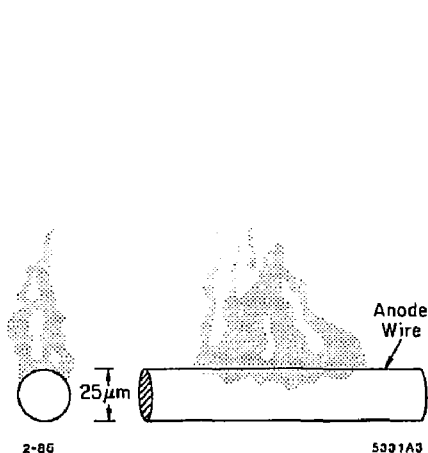
Fig. 3. Monte Carlo prediction of avalanche formation in pure argon. [4]
