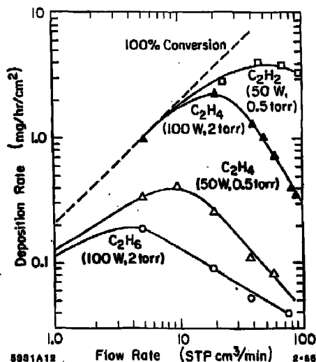
Fig. 15. An effect of a gas flow rate on the polymerisation rate of acetylene, ethylene and ethane in a plasma chemistry environment. [78]
